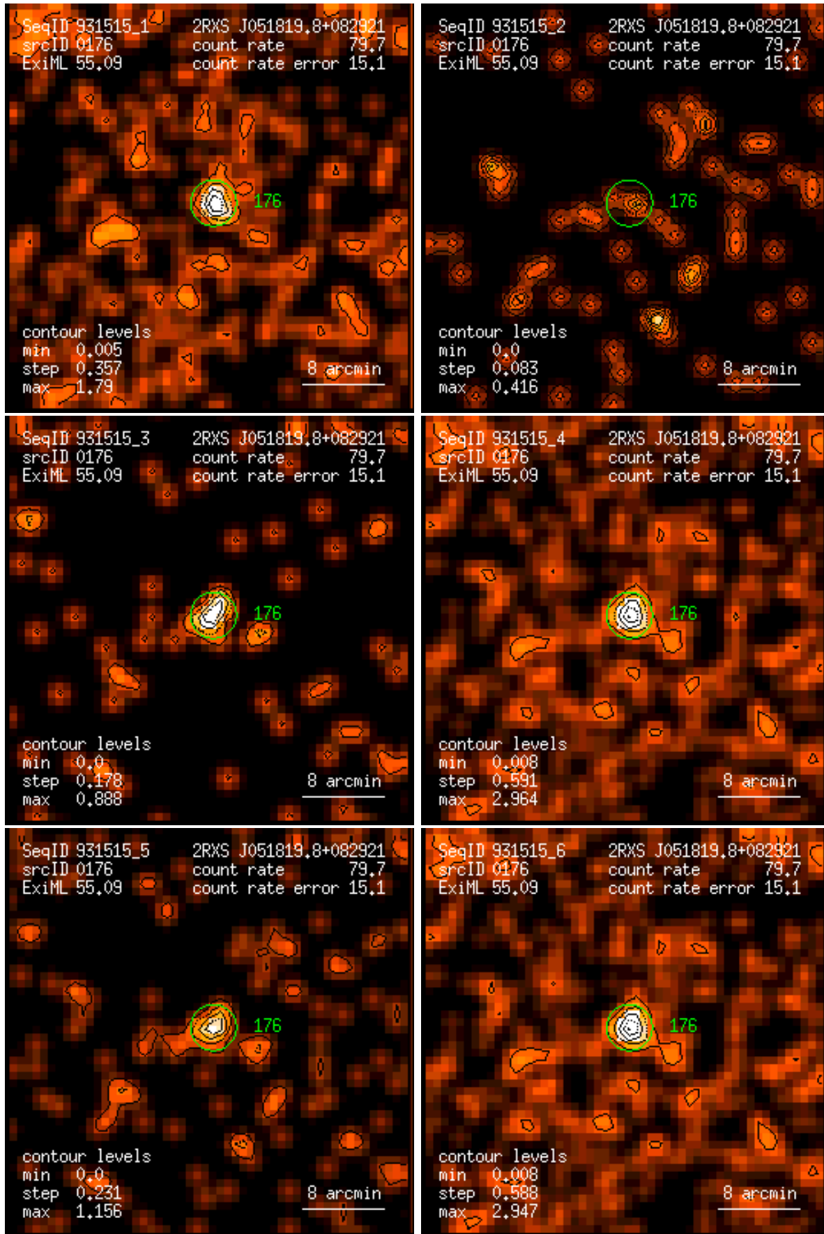
Figure 176: RASS 931515: detection 0176: band rate images, Gaussian filter: (1) PSPC channels 11 – 41, (2) 52 – 90, (3) 91 – 201, (4) 11 – 235, (5) 52 – 201, (6) 11 – 201. Broad band rates in counts/ks. Band rate contour levels in counts/ks/arcmin 2 .
