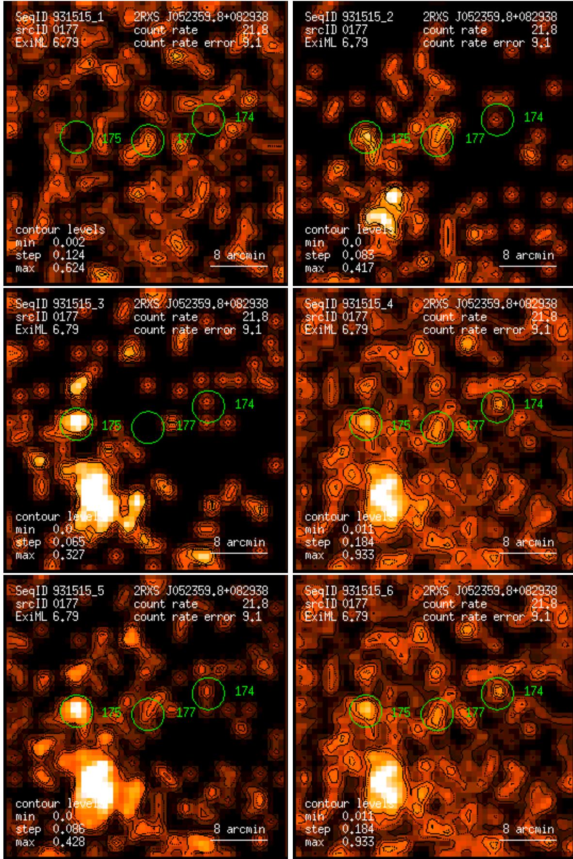
Figure 177: RASS 931515: detection 0177: band rate images, Gaussian filter: (1) PSPC channels 11 – 41, (2) 52 – 90, (3) 91 – 201, (4) 11 – 235, (5) 52 – 201, (6) 11 – 201. Broad band rates in counts/ks. Band rate contour levels in counts/ks/arcmin 2 .
