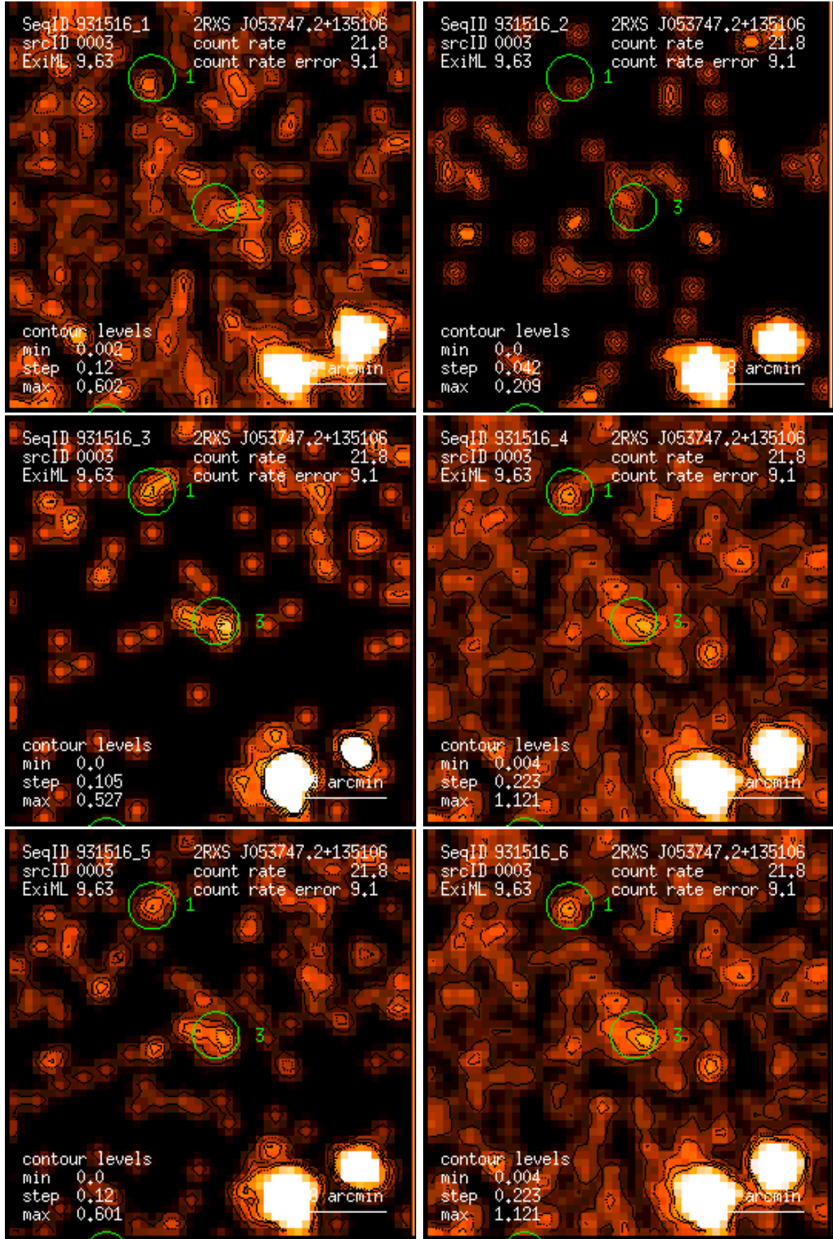
Figure 3: RASS 931516: detection 0003: band rate images, Gaussian filter: (1) PSPC channels 11 – 41, (2) 52 – 90, (3) 91 – 201, (4) 11 – 235, (5) 52 – 201, (6) 11 – 201. Broad band rates in counts/ks. Band rate contour levels in counts/ks/arcmin 2 .
