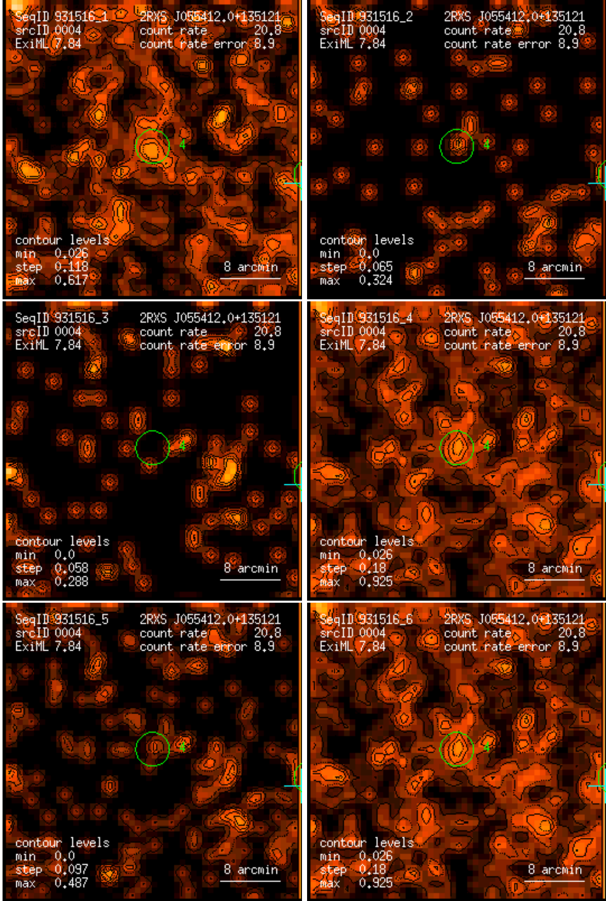
Figure 4: RASS 931516: detection 0004: band rate images, Gaussian filter: (1) PSPC channels 11 – 41, (2) 52 – 90, (3) 91 – 201, (4) 11 – 235, (5) 52 – 201, (6) 11 – 201. Broad band rates in counts/ks. Band rate contour levels in counts/ks/arcmin 2 .
