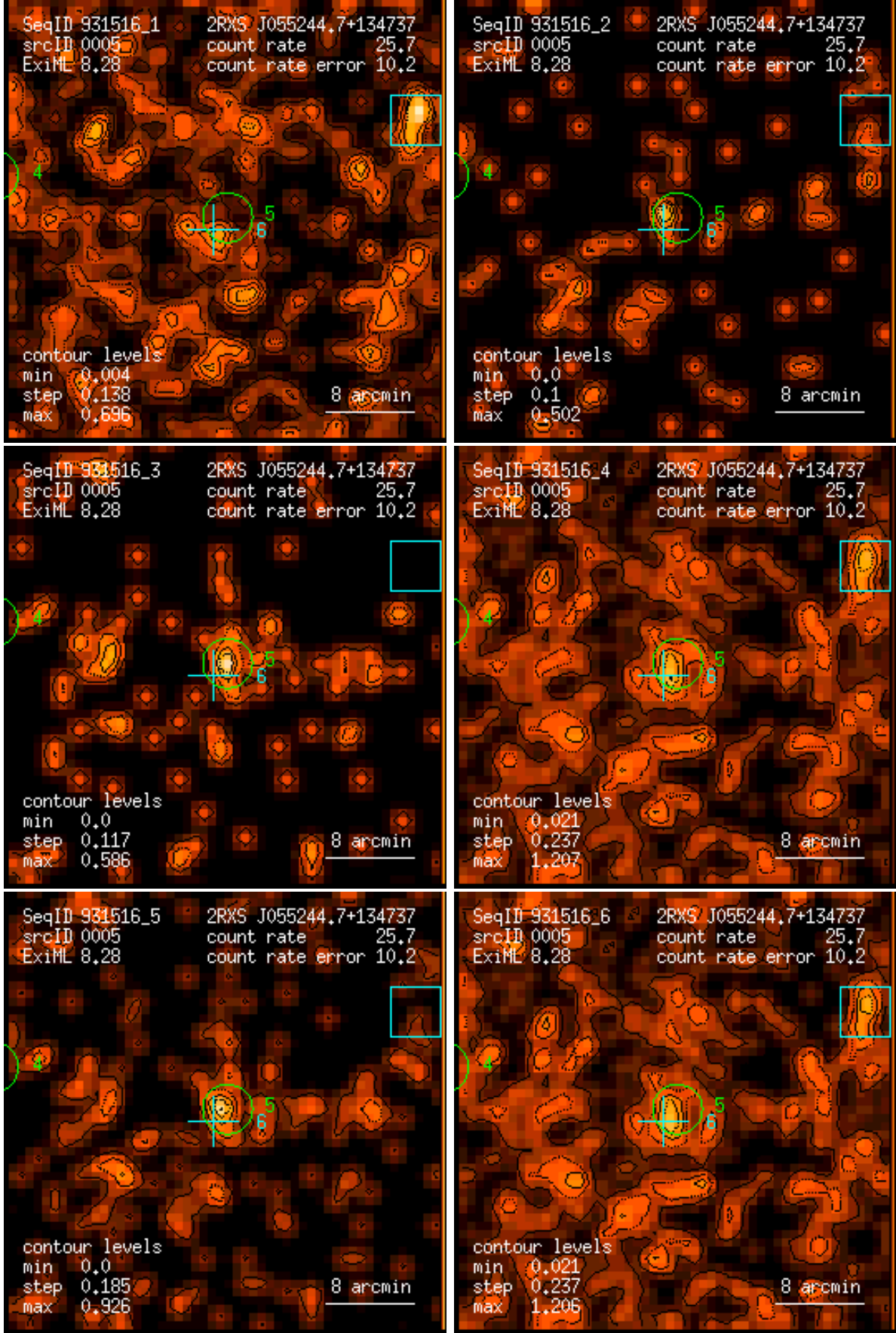
Figure 5: RASS 931516: detection 0005: band rate images, Gaussian filter: (1) PSPC channels 11 – 41, (2) 52 – 90, (3) 91 – 201, (4) 11 – 235, (5) 52 – 201, (6) 11 – 201. Broad band rates in counts/ks. Band rate contour levels in counts/ks/arcmin 2 .
