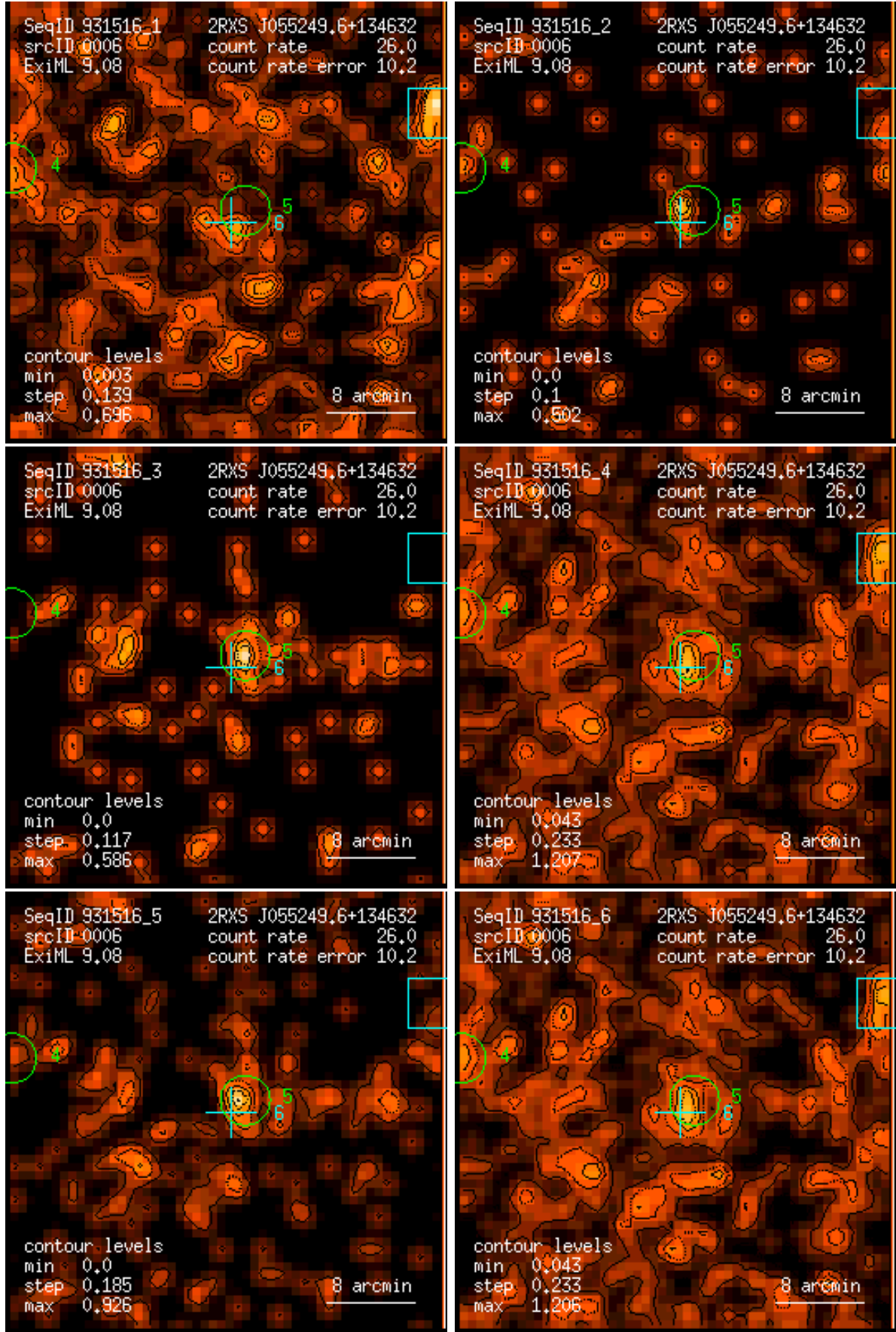
Figure 6: RASS 931516: detection 0006: band rate images, Gaussian filter: (1) PSPC channels 11 – 41, (2) 52 – 90, (3) 91 – 201, (4) 11 – 235, (5) 52 – 201, (6) 11 – 201. Broad band rates in counts/ks. Band rate contour levels in counts/ks/arcmin 2 .
