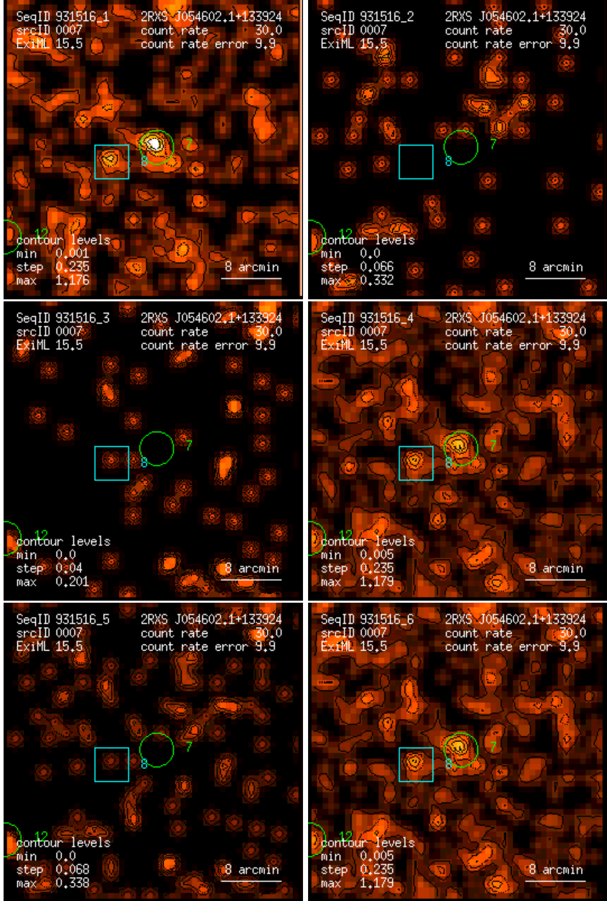
Figure 7: RASS 931516: detection 0007: band rate images, Gaussian filter: (1) PSPC channels 11 – 41, (2) 52 – 90, (3) 91 – 201, (4) 11 – 235, (5) 52 – 201, (6) 11 – 201. Broad band rates in counts/ks. Band rate contour levels in counts/ks/arcmin 2 .
