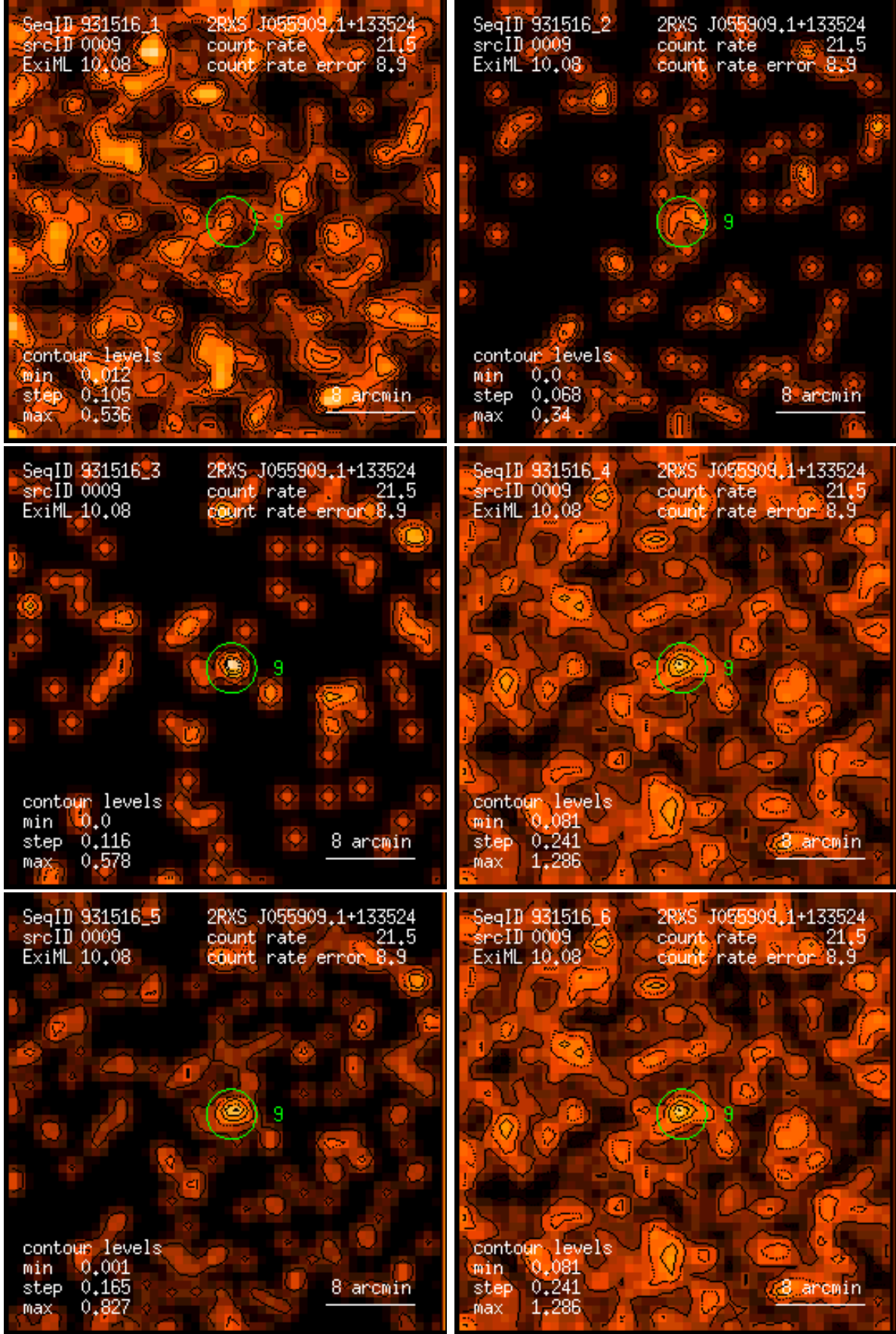
Figure 9: RASS 931516: detection 0009: band rate images, Gaussian filter: (1) PSPC channels 11 – 41, (2) 52 – 90, (3) 91 – 201, (4) 11 – 235, (5) 52 – 201, (6) 11 – 201. Broad band rates in counts/ks. Band rate contour levels in counts/ks/arcmin 2 .
