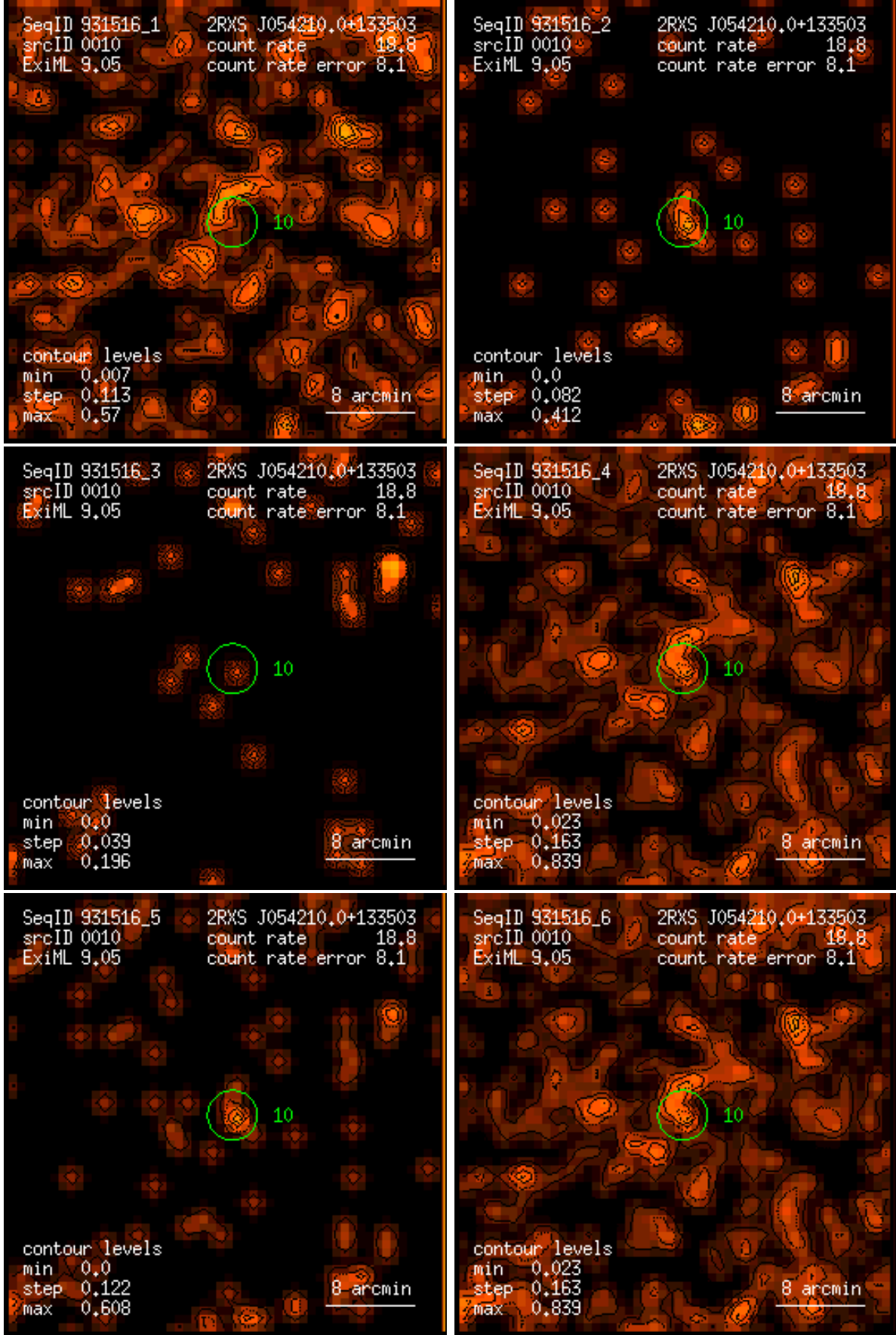
Figure 10: RASS 931516: detection 0010: band rate images, Gaussian filter: (1) PSPC channels 11 – 41, (2) 52 – 90, (3) 91 – 201, (4) 11 – 235, (5) 52 – 201, (6) 11 – 201. Broad band rates in counts/ks. Band rate contour levels in counts/ks/arcmin 2 .
