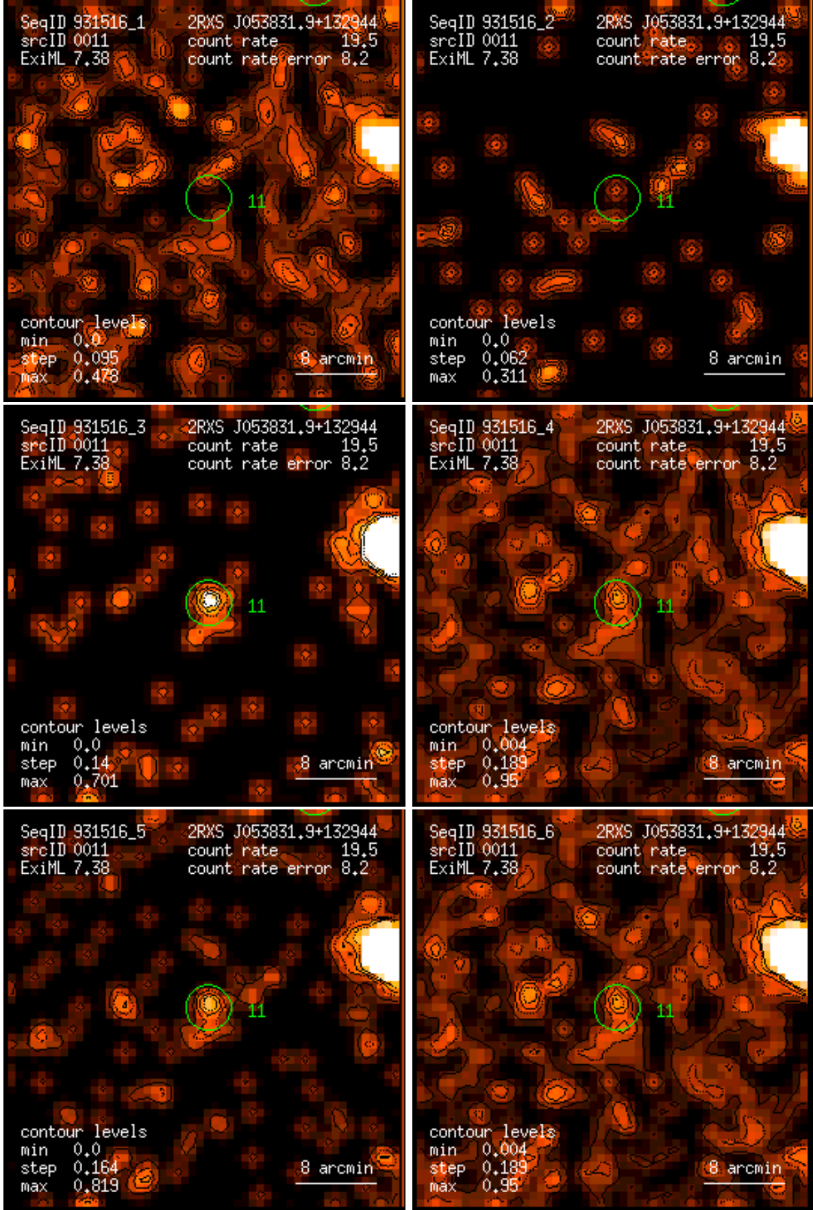
Figure 11: RASS 931516: detection 0011: band rate images, Gaussian filter: (1) PSPC channels 11 – 41, (2) 52 – 90, (3) 91 – 201, (4) 11 – 235, (5) 52 – 201, (6) 11 – 201. Broad band rates in counts/ks. Band rate contour levels in counts/ks/arcmin 2 .
