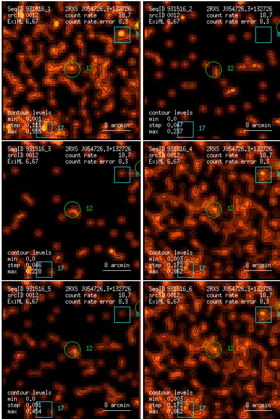
Figure 12: RASS 931516: detection 0012: band rate images, Gaussian filter: (1) PSPC channels 11 – 41, (2) 52 – 90, (3) 91 – 201, (4) 11 – 235, (5) 52 – 201, (6) 11 – 201. Broad band rates in counts/ks. Band rate contour levels in counts/ks/arcmin 2 .
