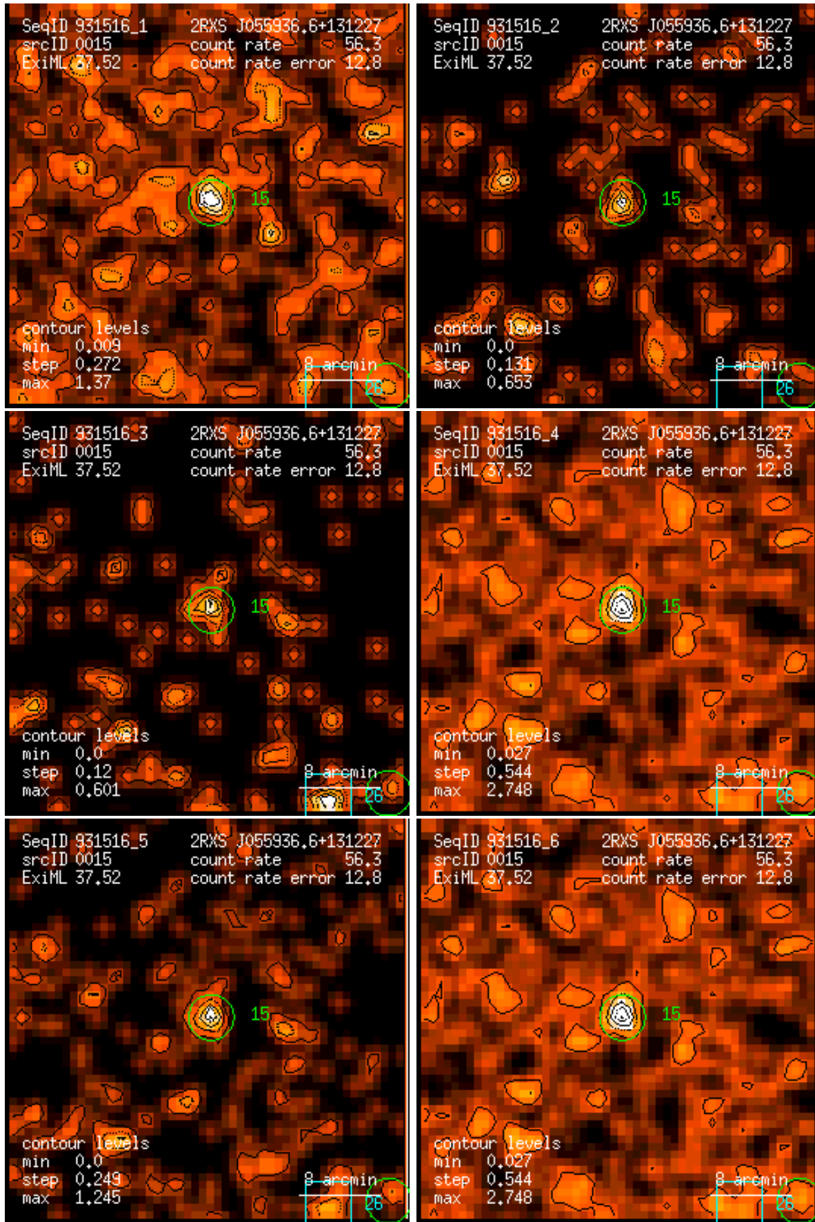
Figure 15: RASS 931516: detection 0015: band rate images, Gaussian filter: (1) PSPC channels 11 – 41, (2) 52 – 90, (3) 91 – 201, (4) 11 – 235, (5) 52 – 201, (6) 11 – 201. Broad band rates in counts/ks. Band rate contour levels in counts/ks/arcmin 2 .
