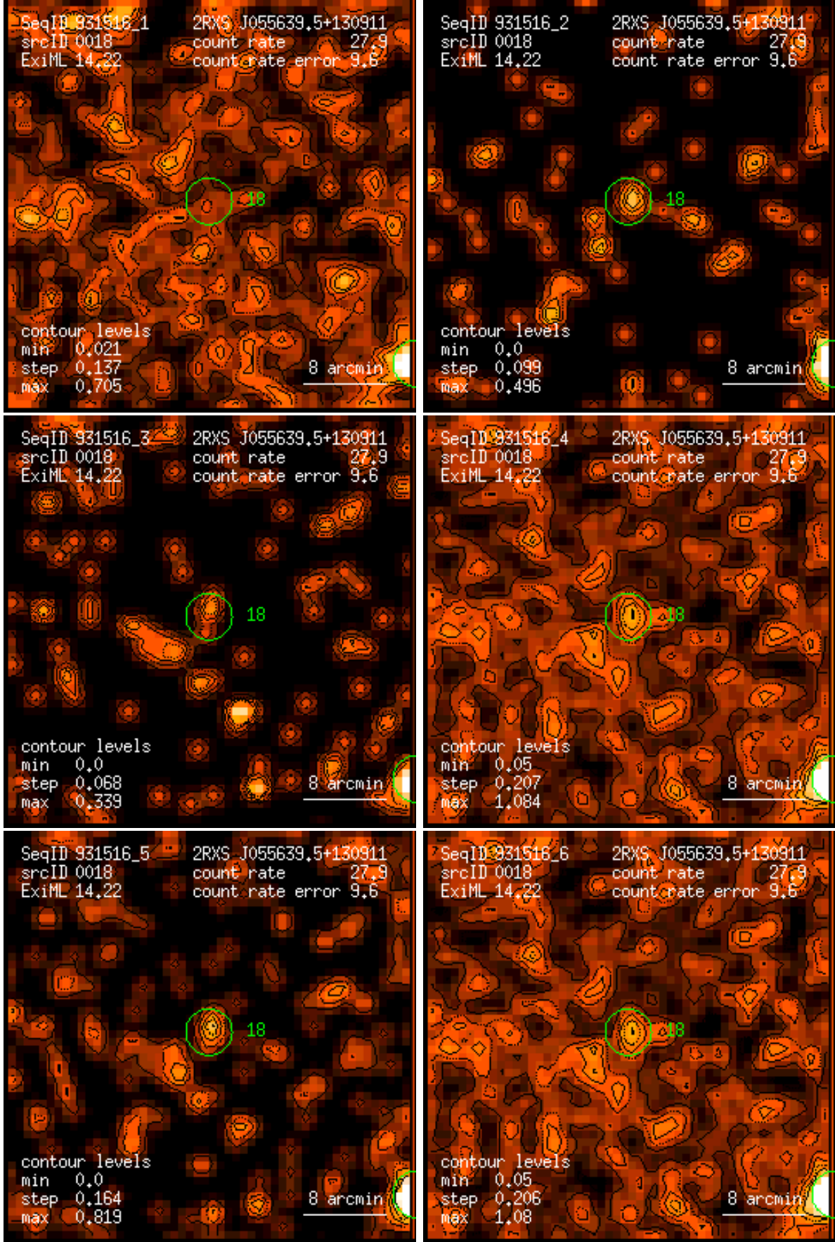
Figure 18: RASS 931516: detection 0018: band rate images, Gaussian filter: (1) PSPC channels 11 – 41, (2) 52 – 90, (3) 91 – 201, (4) 11 – 235, (5) 52 – 201, (6) 11 – 201. Broad band rates in counts/ks. Band rate contour levels in counts/ks/arcmin 2 .
