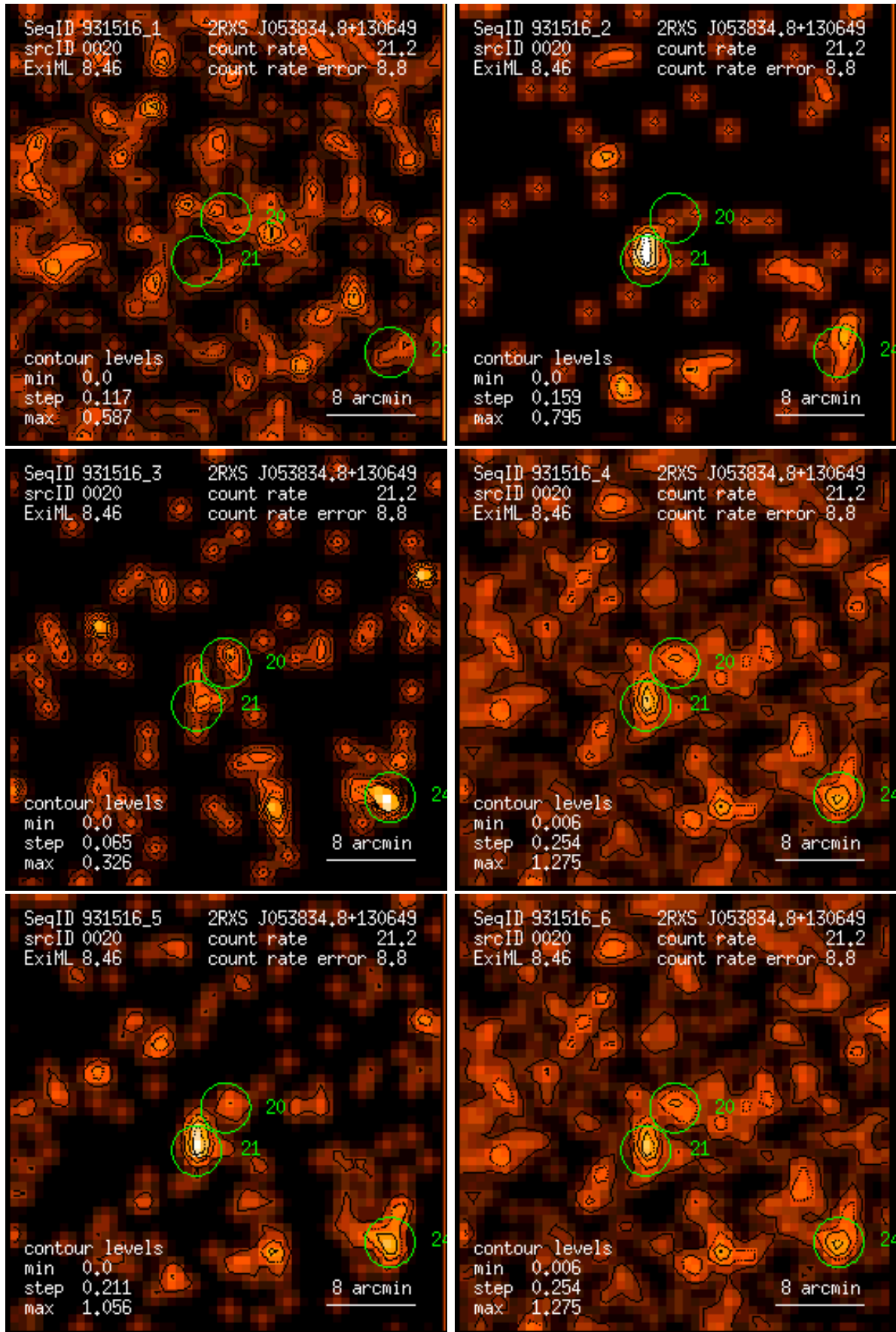
Figure 20: RASS 931516: detection 0020: band rate images, Gaussian filter: (1) PSPC channels 11 – 41, (2) 52 – 90, (3) 91 – 201, (4) 11 – 235, (5) 52 – 201, (6) 11 – 201. Broad band rates in counts/ks. Band rate contour levels in counts/ks/arcmin 2 .
