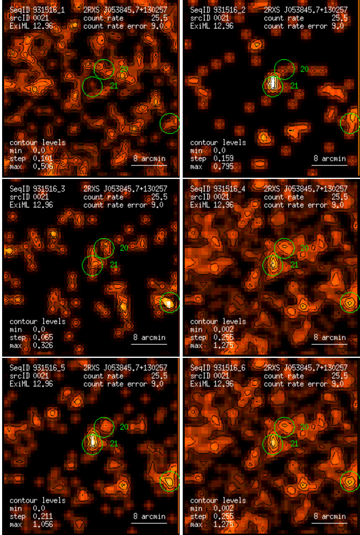
Figure 21: RASS 931516: detection 0021: band rate images, Gaussian filter: (1) PSPC channels 11 – 41, (2) 52 – 90, (3) 91 – 201, (4) 11 – 235, (5) 52 – 201, (6) 11 – 201. Broad band rates in counts/ks. Band rate contour levels in counts/ks/arcmin 2 .
