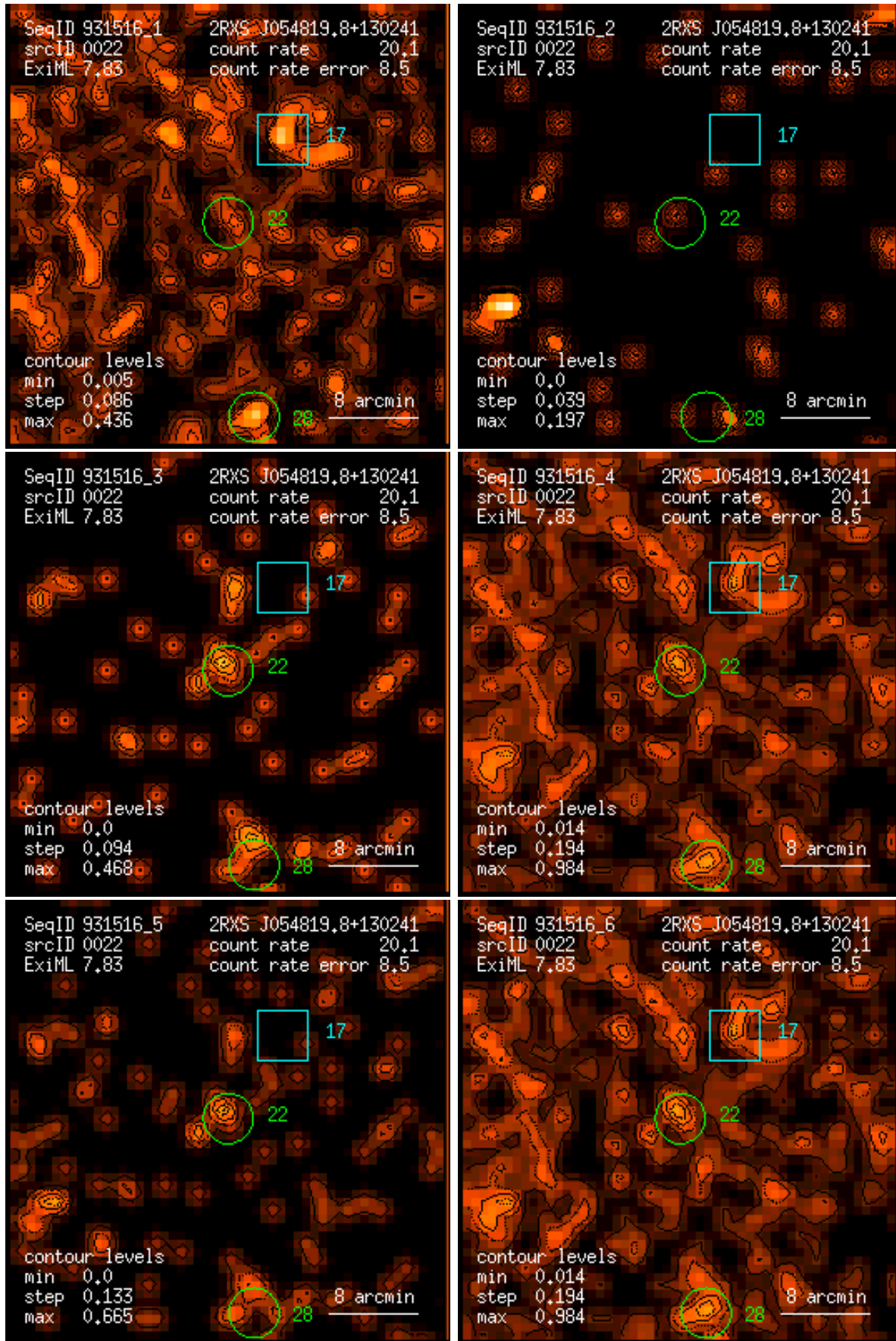
Figure 22: RASS 931516: detection 0022: band rate images, Gaussian filter: (1) PSPC channels 11 – 41, (2) 52 – 90, (3) 91 – 201, (4) 11 – 235, (5) 52 – 201, (6) 11 – 201. Broad band rates in counts/ks. Band rate contour levels in counts/ks/arcmin 2 .
