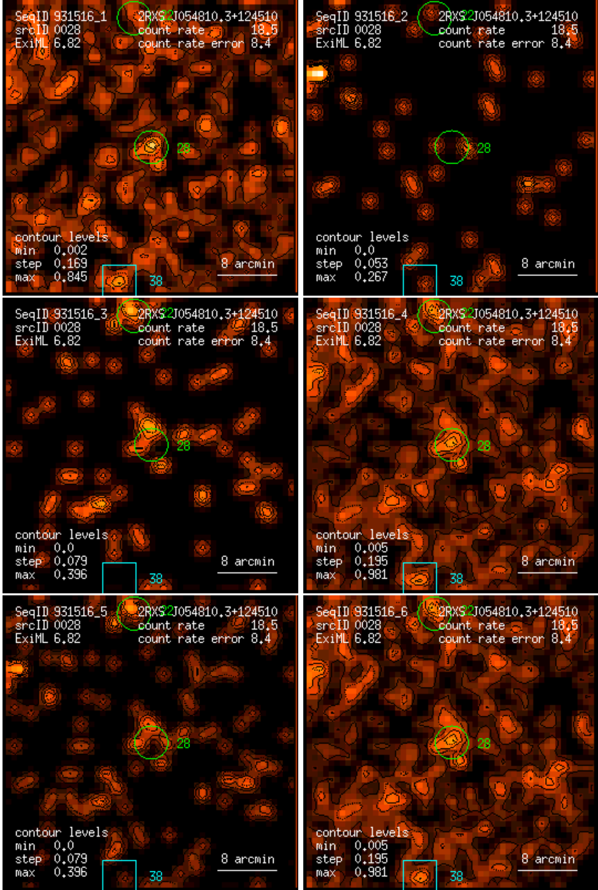
Figure 28: RASS 931516: detection 0028: band rate images, Gaussian filter: (1) PSPC channels 11 – 41, (2) 52 – 90, (3) 91 – 201, (4) 11 – 235, (5) 52 – 201, (6) 11 – 201. Broad band rates in counts/ks. Band rate contour levels in counts/ks/arcmin 2 .
