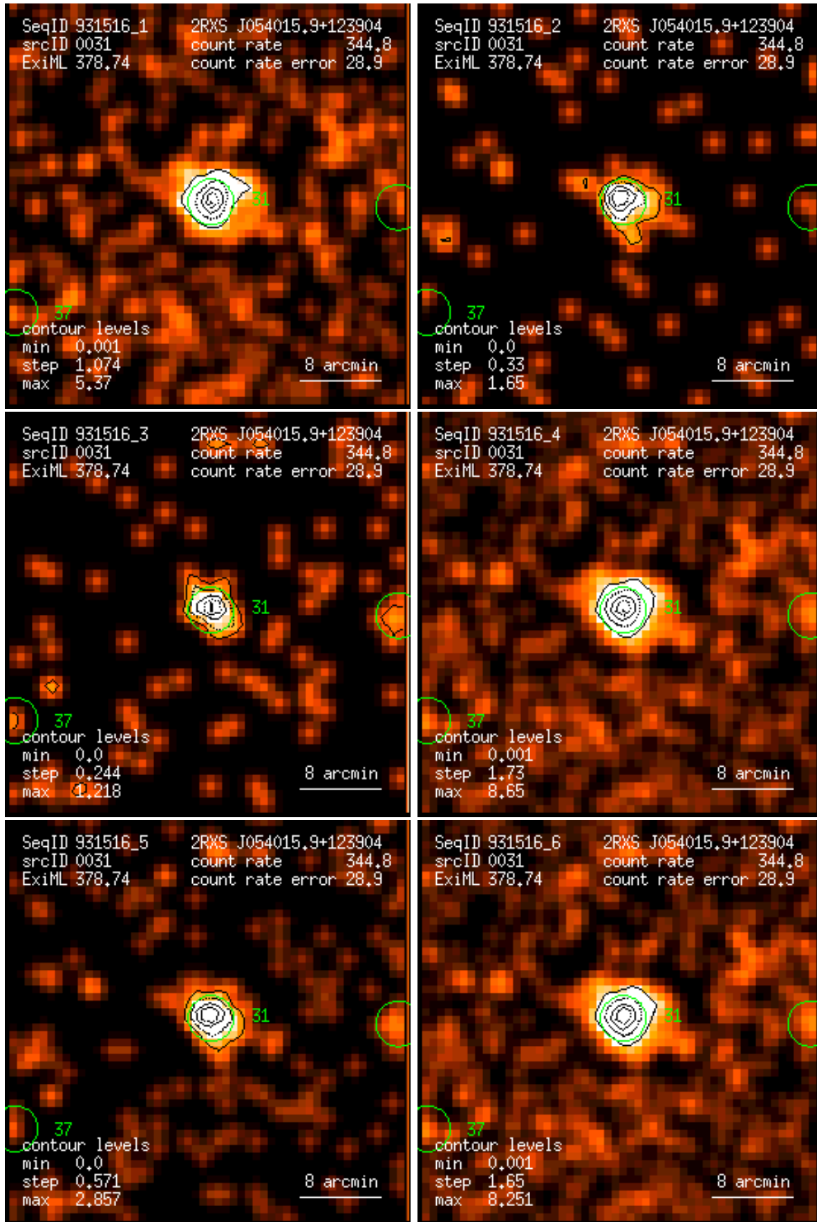
Figure 31: RASS 931516: detection 0031: band rate images, Gaussian filter: (1) PSPC channels 11 – 41, (2) 52 – 90, (3) 91 – 201, (4) 11 – 235, (5) 52 – 201, (6) 11 – 201. Broad band rates in counts/ks. Band rate contour levels in counts/ks/arcmin 2 .
