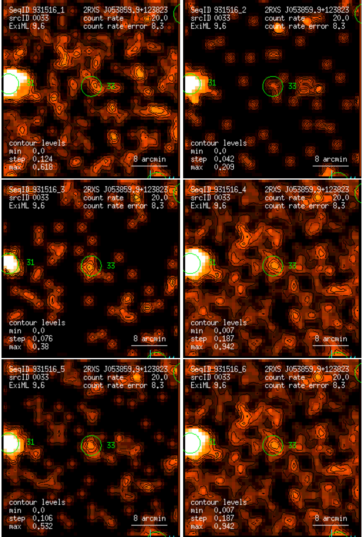
Figure 33: RASS 931516: detection 0033: band rate images, Gaussian filter: (1) PSPC channels 11 – 41, (2) 52 – 90, (3) 91 – 201, (4) 11 – 235, (5) 52 – 201, (6) 11 – 201. Broad band rates in counts/ks. Band rate contour levels in counts/ks/arcmin 2 .
