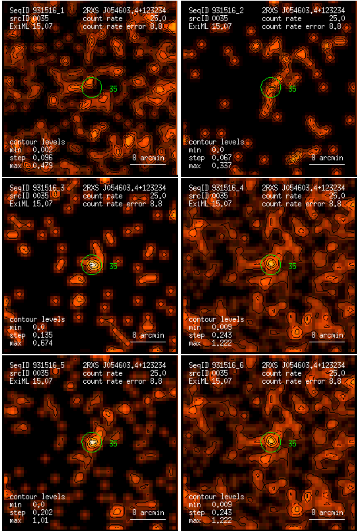
Figure 35: RASS 931516: detection 0035: band rate images, Gaussian filter: (1) PSPC channels 11 – 41, (2) 52 – 90, (3) 91 – 201, (4) 11 – 235, (5) 52 – 201, (6) 11 – 201. Broad band rates in counts/ks. Band rate contour levels in counts/ks/arcmin 2 .
