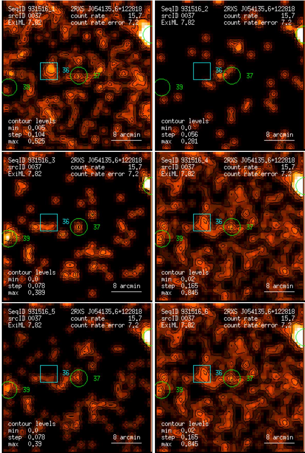
Figure 37: RASS 931516: detection 0037: band rate images, Gaussian filter: (1) PSPC channels 11 – 41, (2) 52 – 90, (3) 91 – 201, (4) 11 – 235, (5) 52 – 201, (6) 11 – 201. Broad band rates in counts/ks. Band rate contour levels in counts/ks/arcmin 2 .
