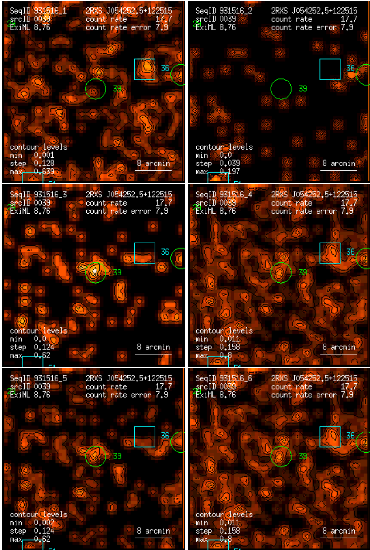
Figure 39: RASS 931516: detection 0039: band rate images, Gaussian filter: (1) PSPC channels 11 – 41, (2) 52 – 90, (3) 91 – 201, (4) 11 – 235, (5) 52 – 201, (6) 11 – 201. Broad band rates in counts/ks. Band rate contour levels in counts/ks/arcmin 2 .
