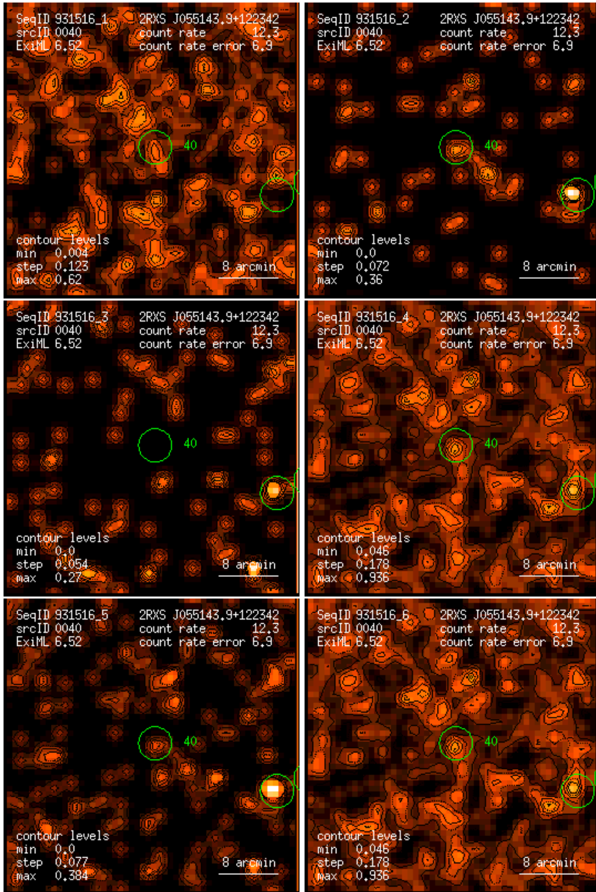
Figure 40: RASS 931516: detection 0040: band rate images, Gaussian filter: (1) PSPC channels 11 – 41, (2) 52 – 90, (3) 91 – 201, (4) 11 – 235, (5) 52 – 201, (6) 11 – 201. Broad band rates in counts/ks. Band rate contour levels in counts/ks/arcmin 2 .
