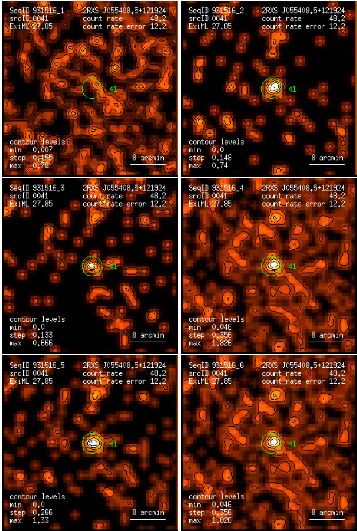
Figure 41: RASS 931516: detection 0041: band rate images, Gaussian filter: (1) PSPC channels 11 – 41, (2) 52 – 90, (3) 91 – 201, (4) 11 – 235, (5) 52 – 201, (6) 11 – 201. Broad band rates in counts/ks. Band rate contour levels in counts/ks/arcmin 2 .
