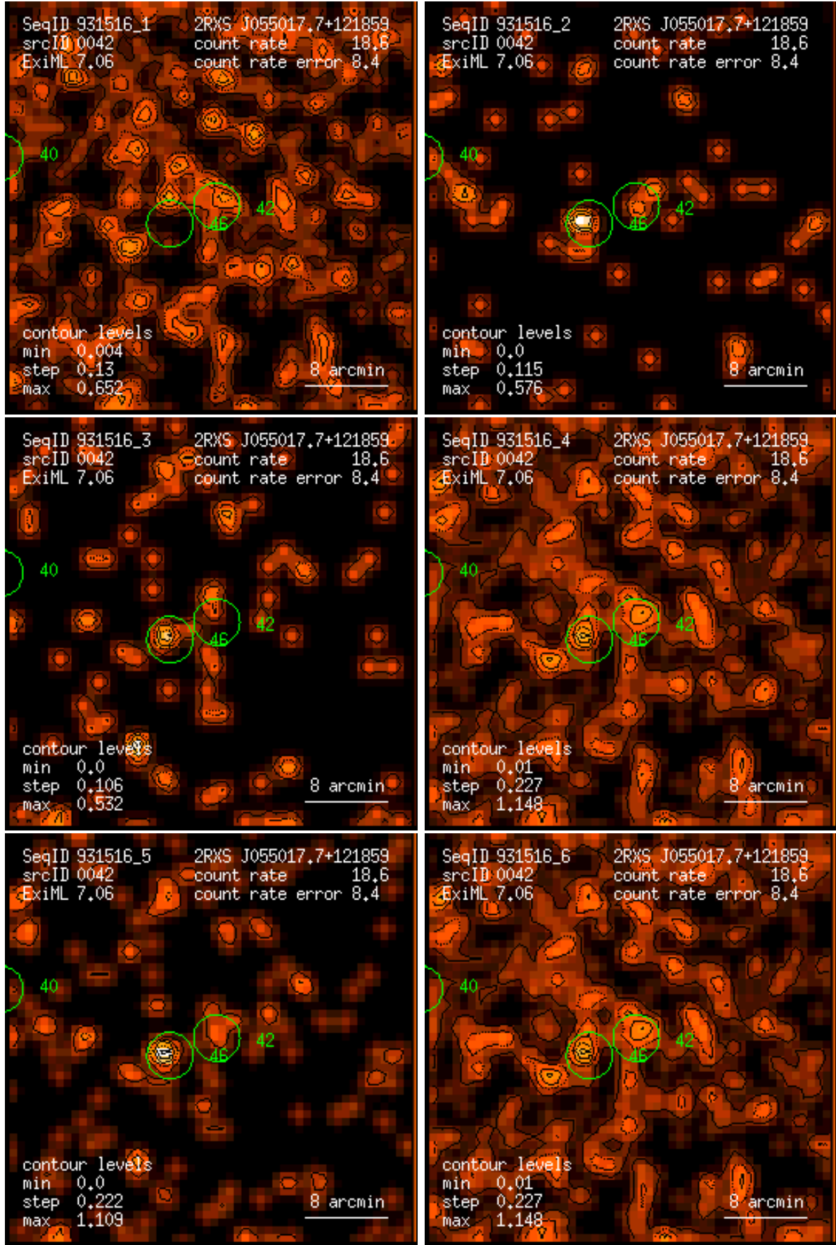
Figure 42: RASS 931516: detection 0042: band rate images, Gaussian filter: (1) PSPC channels 11 – 41, (2) 52 – 90, (3) 91 – 201, (4) 11 – 235, (5) 52 – 201, (6) 11 – 201. Broad band rates in counts/ks. Band rate contour levels in counts/ks/arcmin 2 .
