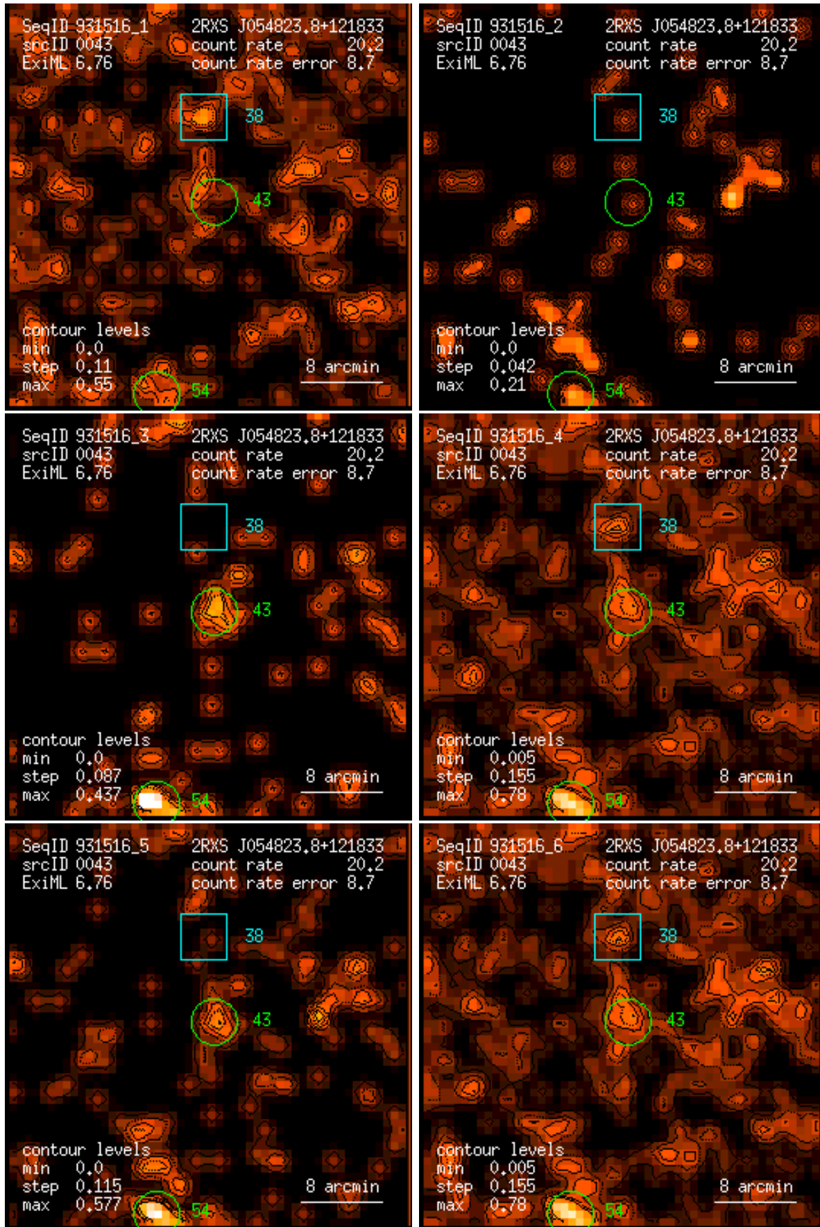
Figure 43: RASS 931516: detection 0043: band rate images, Gaussian filter: (1) PSPC channels 11 – 41, (2) 52 – 90, (3) 91 – 201, (4) 11 – 235, (5) 52 – 201, (6) 11 – 201. Broad band rates in counts/ks. Band rate contour levels in counts/ks/arcmin 2 .
