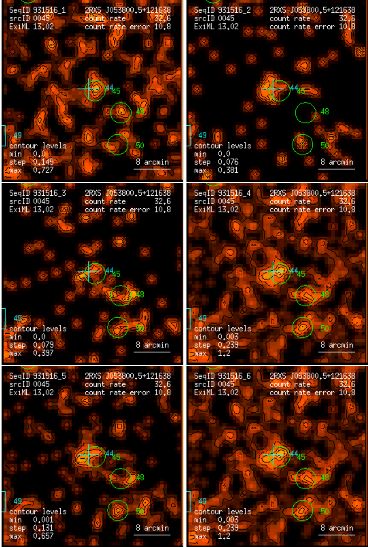
Figure 45: RASS 931516: detection 0045: band rate images, Gaussian filter: (1) PSPC channels 11 – 41, (2) 52 – 90, (3) 91 – 201, (4) 11 – 235, (5) 52 – 201, (6) 11 – 201. Broad band rates in counts/ks. Band rate contour levels in counts/ks/arcmin 2 .
