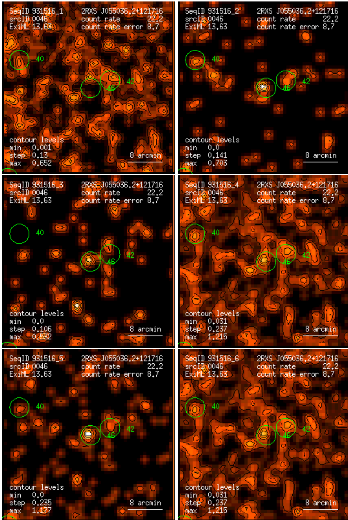
Figure 46: RASS 931516: detection 0046: band rate images, Gaussian filter: (1) PSPC channels 11 – 41, (2) 52 – 90, (3) 91 – 201, (4) 11 – 235, (5) 52 – 201, (6) 11 – 201. Broad band rates in counts/ks. Band rate contour levels in counts/ks/arcmin 2 .
