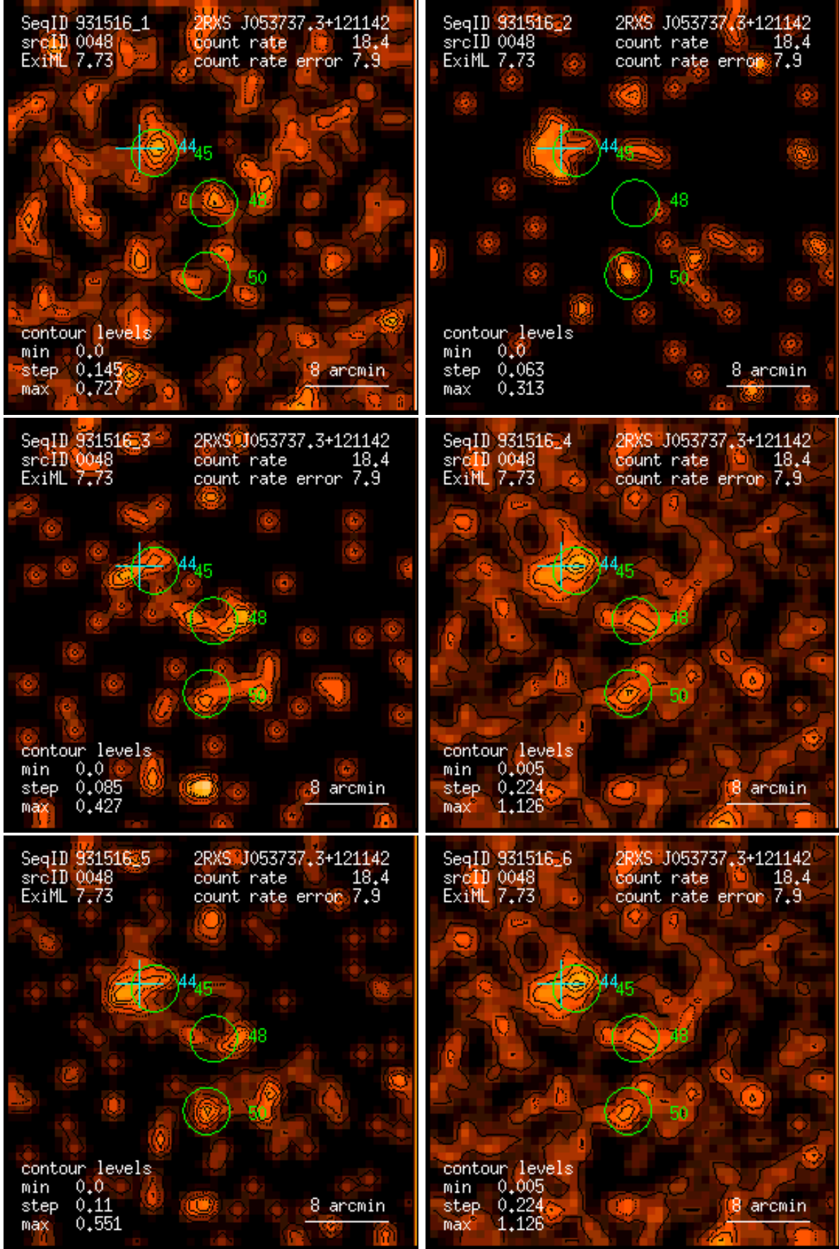
Figure 48: RASS 931516: detection 0048: band rate images, Gaussian filter: (1) PSPC channels 11 – 41, (2) 52 – 90, (3) 91 – 201, (4) 11 – 235, (5) 52 – 201, (6) 11 – 201. Broad band rates in counts/ks. Band rate contour levels in counts/ks/arcmin 2 .
