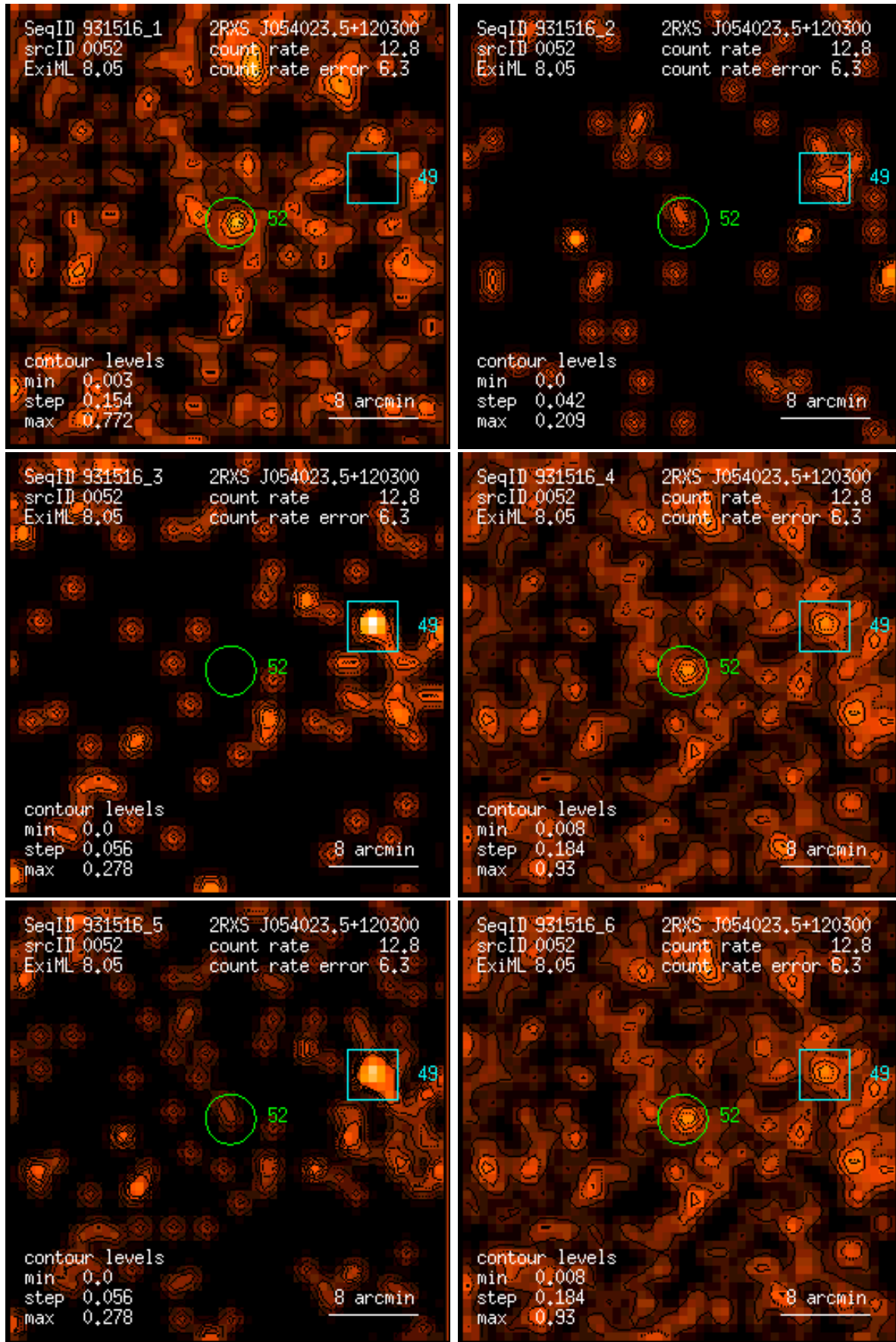
Figure 52: RASS 931516: detection 0052: band rate images, Gaussian filter: (1) PSPC channels 11 – 41, (2) 52 – 90, (3) 91 – 201, (4) 11 – 235, (5) 52 – 201, (6) 11 – 201. Broad band rates in counts/ks. Band rate contour levels in counts/ks/arcmin 2 .
