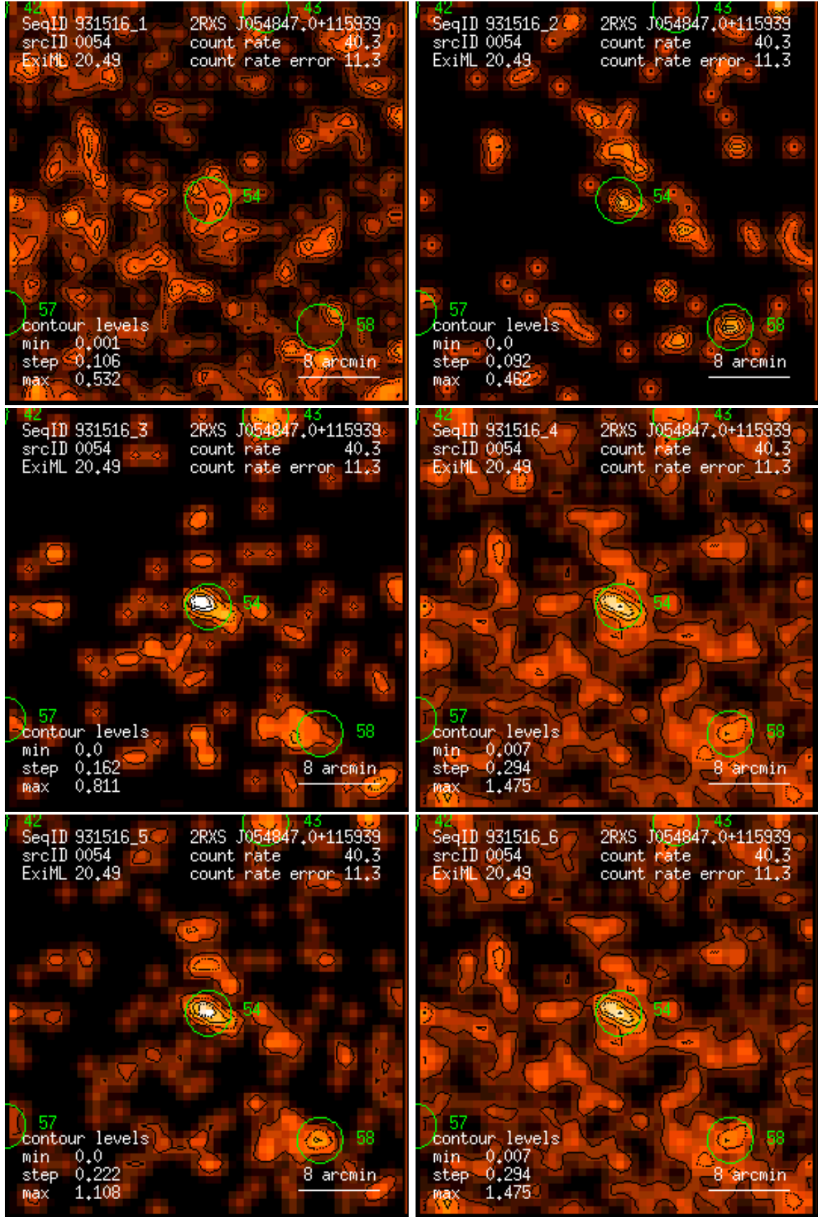
Figure 54: RASS 931516: detection 0054: band rate images, Gaussian filter: (1) PSPC channels 11 – 41, (2) 52 – 90, (3) 91 – 201, (4) 11 – 235, (5) 52 – 201, (6) 11 – 201. Broad band rates in counts/ks. Band rate contour levels in counts/ks/arcmin 2 .
