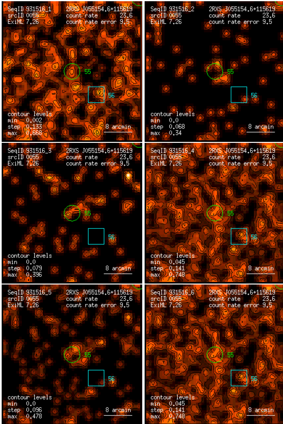
Figure 55: RASS 931516: detection 0055: band rate images, Gaussian filter: (1) PSPC channels 11 – 41, (2) 52 – 90, (3) 91 – 201, (4) 11 – 235, (5) 52 – 201, (6) 11 – 201. Broad band rates in counts/ks. Band rate contour levels in counts/ks/arcmin 2 .
