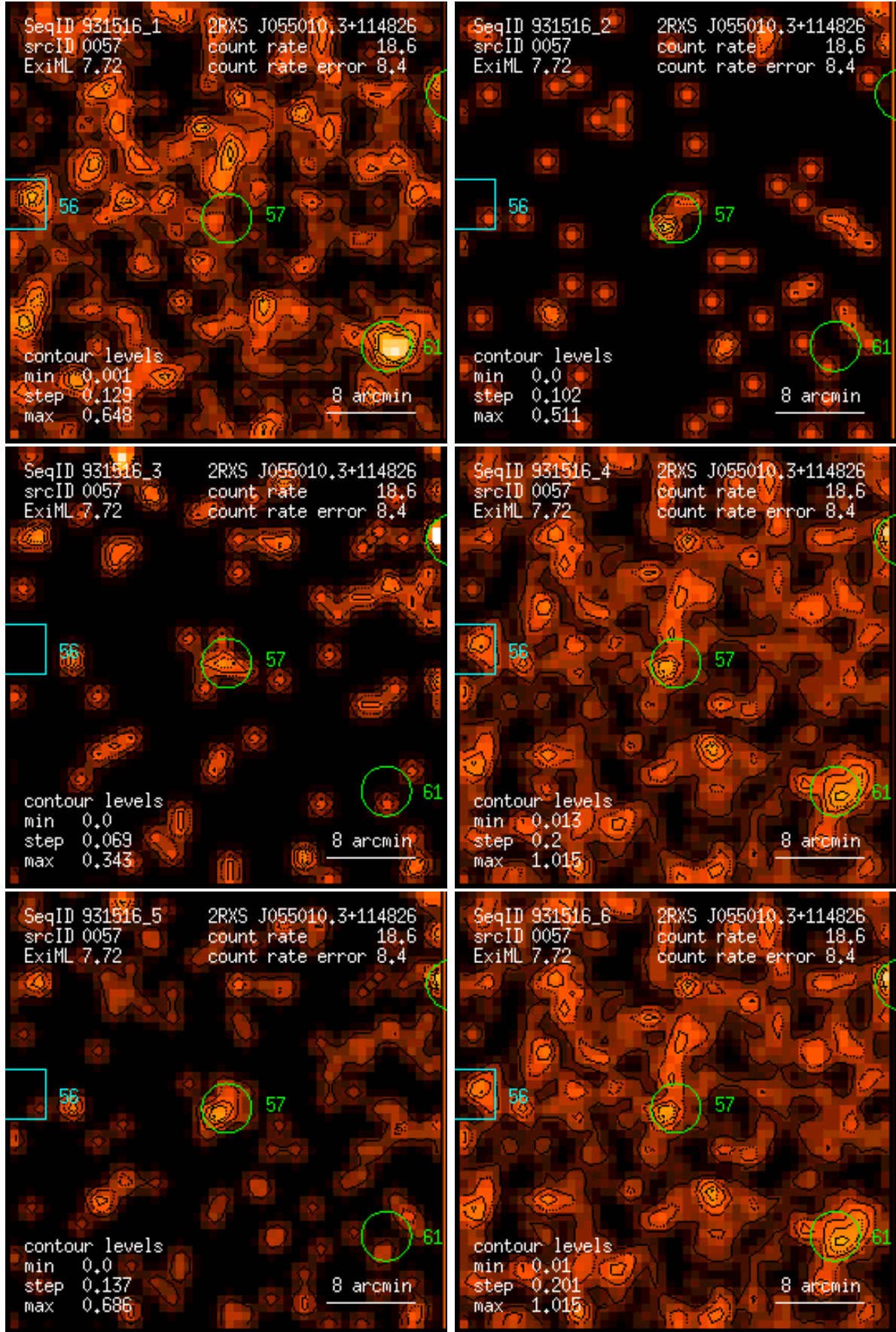
Figure 57: RASS 931516: detection 0057: band rate images, Gaussian filter: (1) PSPC channels 11 – 41, (2) 52 – 90, (3) 91 – 201, (4) 11 – 235, (5) 52 – 201, (6) 11 – 201. Broad band rates in counts/ks. Band rate contour levels in counts/ks/arcmin 2 .
