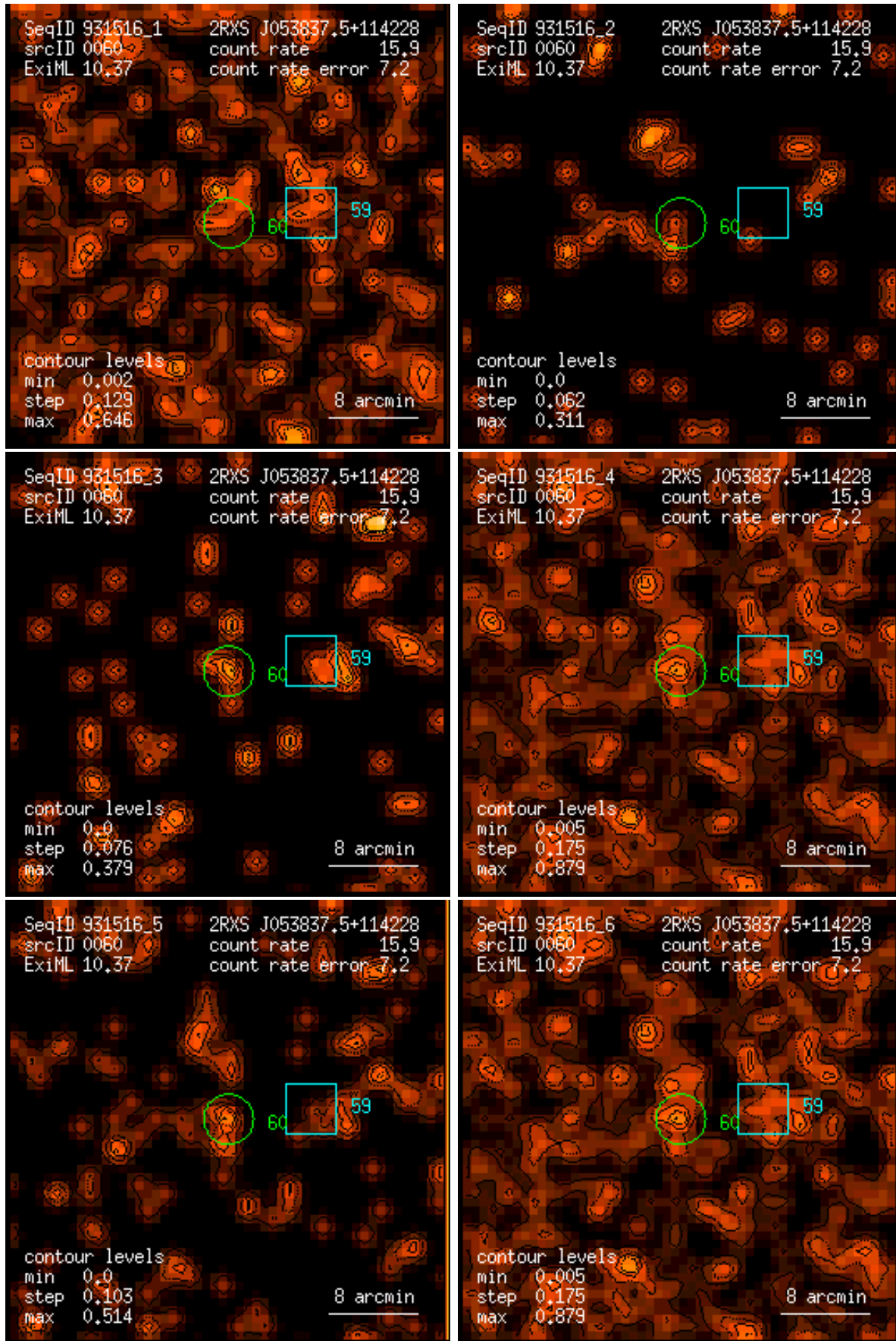
Figure 60: RASS 931516: detection 0060: band rate images, Gaussian filter: (1) PSPC channels 11 – 41, (2) 52 – 90, (3) 91 – 201, (4) 11 – 235, (5) 52 – 201, (6) 11 – 201. Broad band rates in counts/ks. Band rate contour levels in counts/ks/arcmin 2 .
