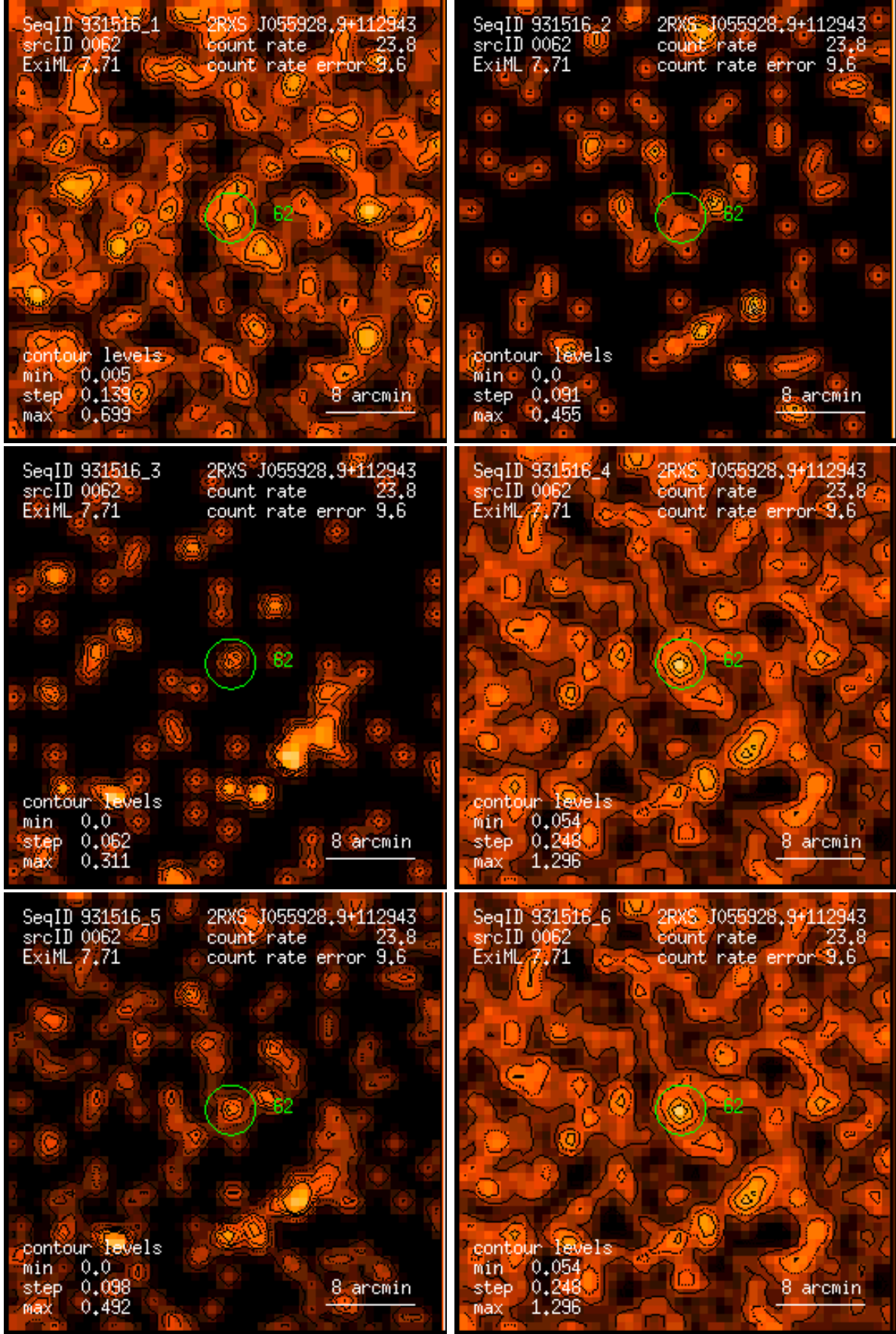
Figure 62: RASS 931516: detection 0062: band rate images, Gaussian filter: (1) PSPC channels 11 – 41, (2) 52 – 90, (3) 91 – 201, (4) 11 – 235, (5) 52 – 201, (6) 11 – 201. Broad band rates in counts/ks. Band rate contour levels in counts/ks/arcmin 2 .
