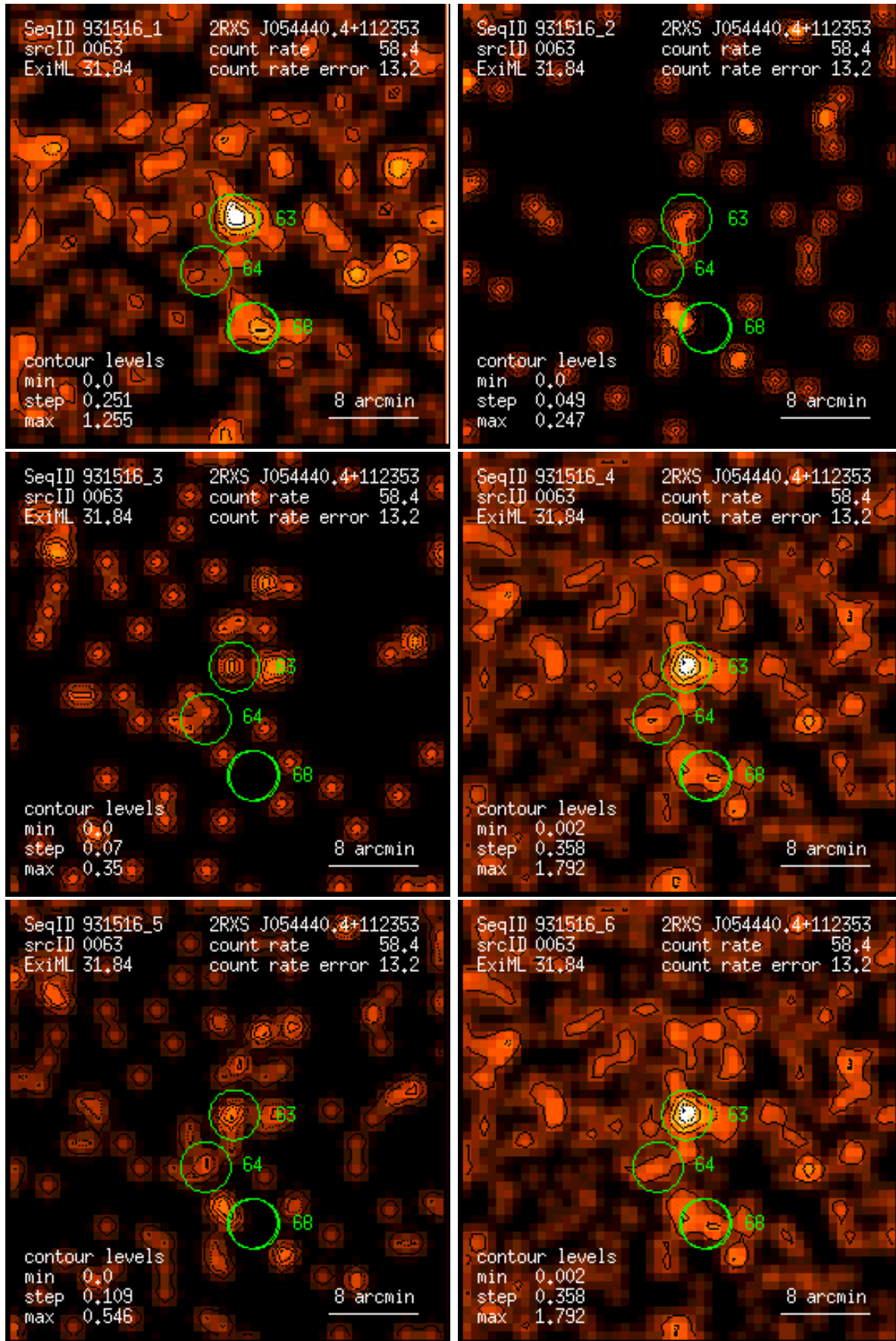
Figure 63: RASS 931516: detection 0063: band rate images, Gaussian filter: (1) PSPC channels 11 – 41, (2) 52 – 90, (3) 91 – 201, (4) 11 – 235, (5) 52 – 201, (6) 11 – 201. Broad band rates in counts/ks. Band rate contour levels in counts/ks/arcmin 2 .
