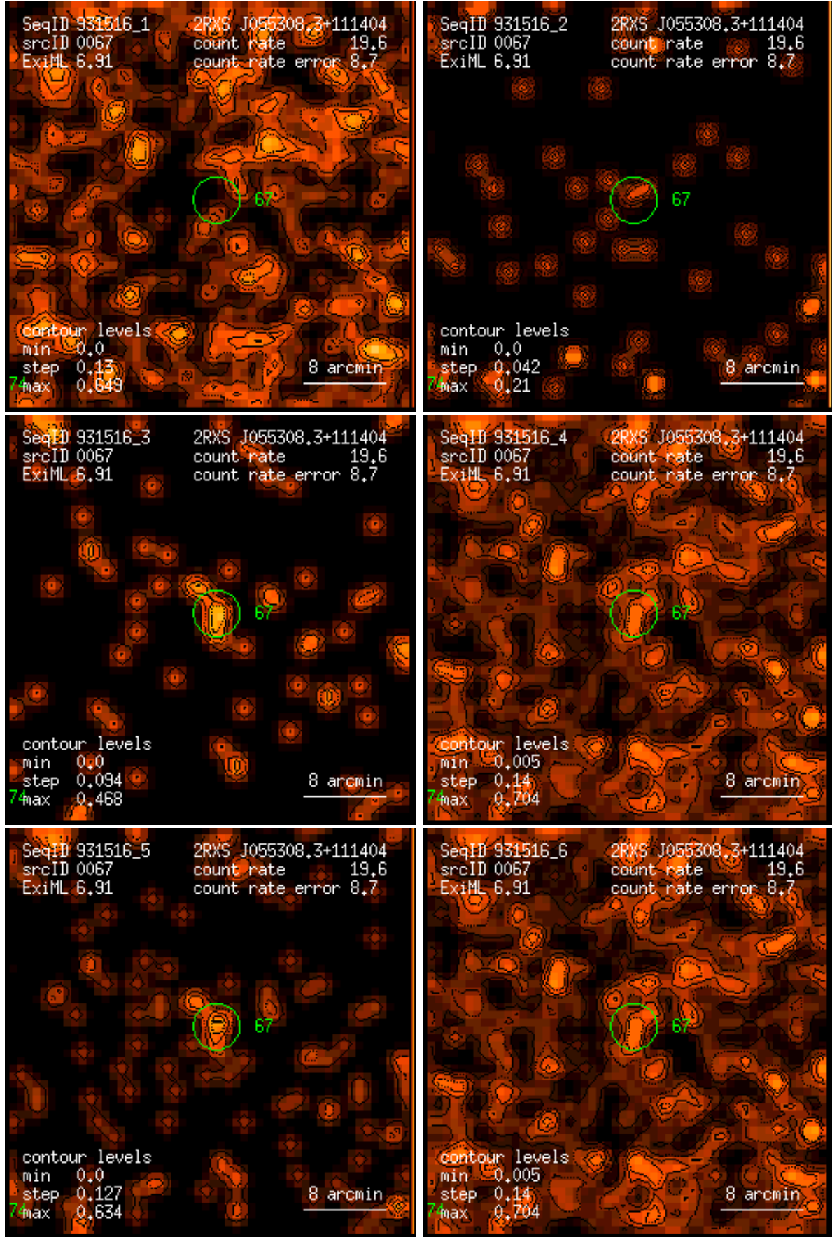
Figure 67: RASS 931516: detection 0067: band rate images, Gaussian filter: (1) PSPC channels 11 – 41, (2) 52 – 90, (3) 91 – 201, (4) 11 – 235, (5) 52 – 201, (6) 11 – 201. Broad band rates in counts/ks. Band rate contour levels in counts/ks/arcmin 2 .
