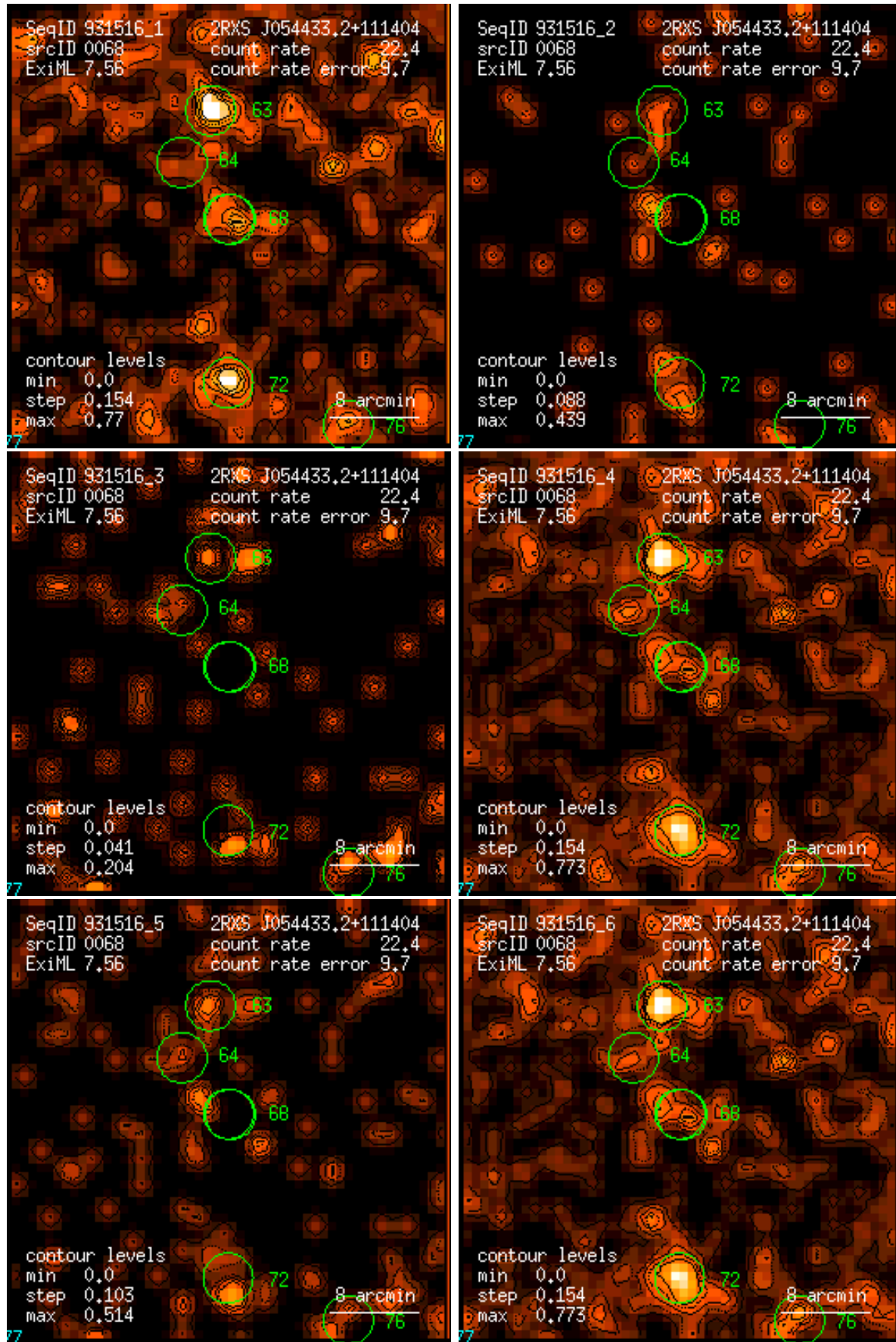
Figure 68: RASS 931516: detection 0068: band rate images, Gaussian filter: (1) PSPC channels 11 – 41, (2) 52 – 90, (3) 91 – 201, (4) 11 – 235, (5) 52 – 201, (6) 11 – 201. Broad band rates in counts/ks. Band rate contour levels in counts/ks/arcmin 2 .
