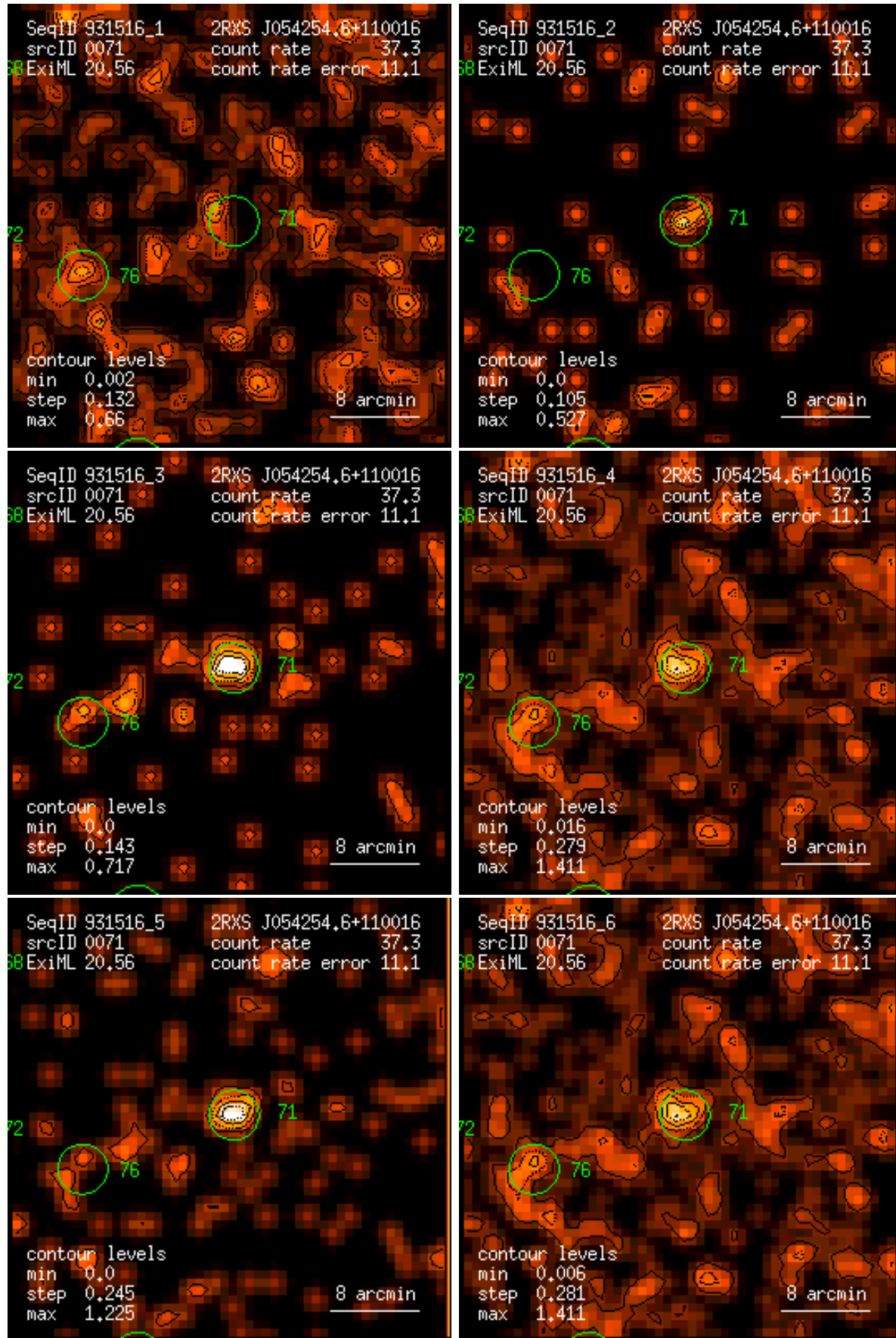
Figure 71: RASS 931516: detection 0071: band rate images, Gaussian filter: (1) PSPC channels 11 – 41, (2) 52 – 90, (3) 91 – 201, (4) 11 – 235, (5) 52 – 201, (6) 11 – 201. Broad band rates in counts/ks. Band rate contour levels in counts/ks/arcmin 2 .
