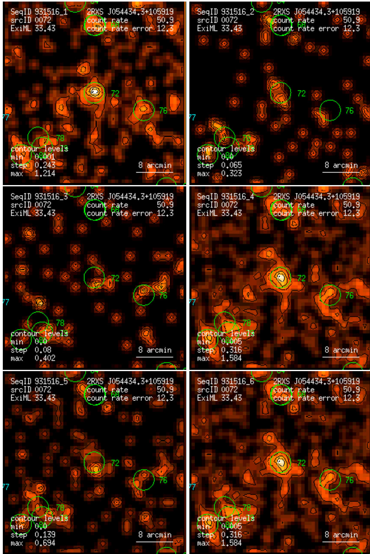
Figure 72: RASS 931516: detection 0072: band rate images, Gaussian filter: (1) PSPC channels 11 – 41, (2) 52 – 90, (3) 91 – 201, (4) 11 – 235, (5) 52 – 201, (6) 11 – 201. Broad band rates in counts/ks. Band rate contour levels in counts/ks/arcmin 2 .
