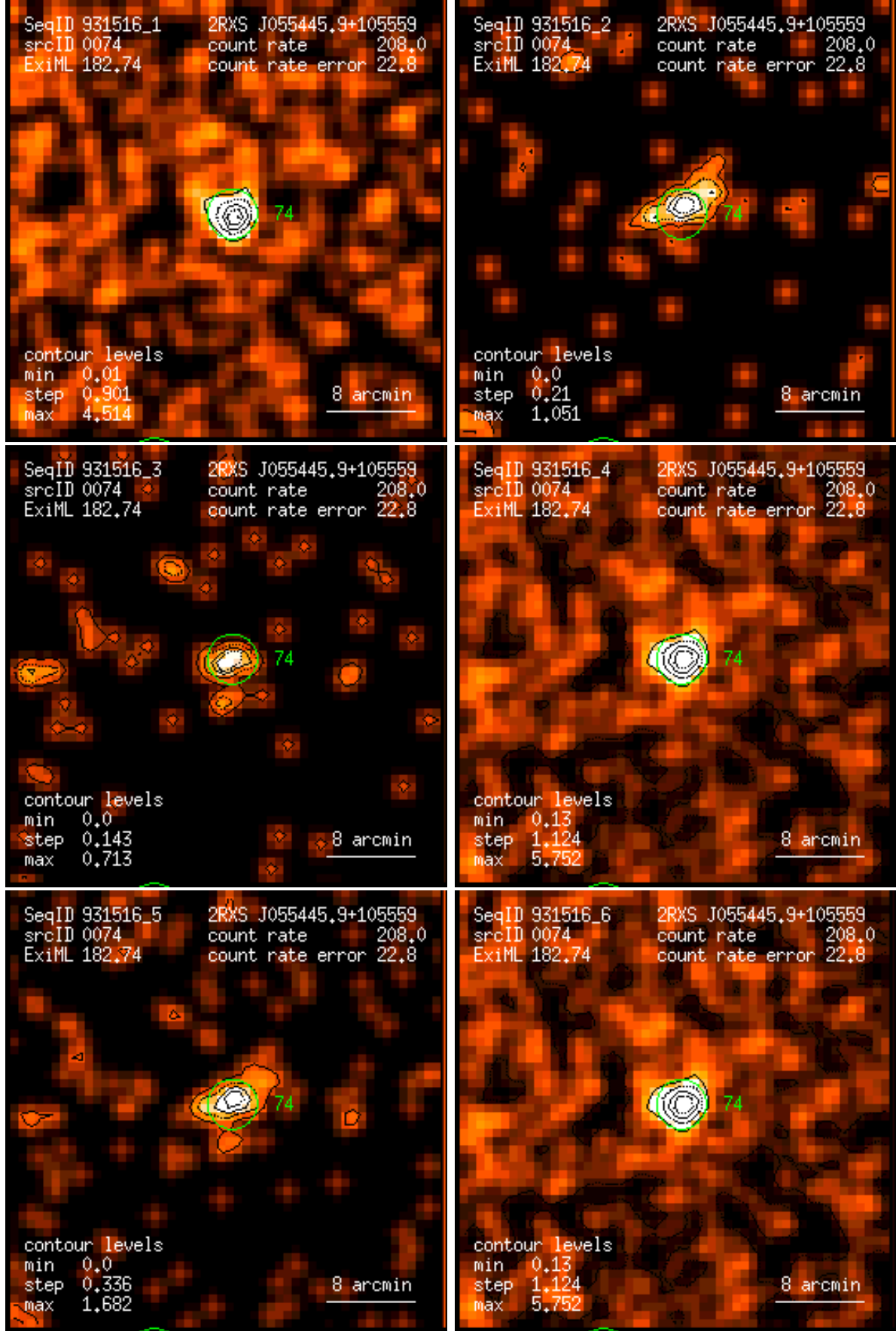
Figure 74: RASS 931516: detection 0074: band rate images, Gaussian filter: (1) PSPC channels 11 – 41, (2) 52 – 90, (3) 91 – 201, (4) 11 – 235, (5) 52 – 201, (6) 11 – 201. Broad band rates in counts/ks. Band rate contour levels in counts/ks/arcmin 2 .
