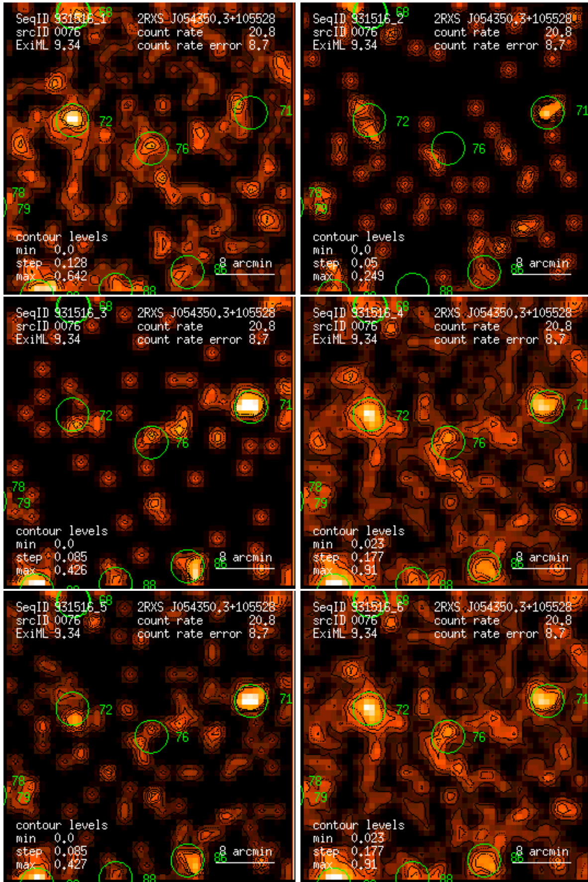
Figure 76: RASS 931516: detection 0076: band rate images, Gaussian filter: (1) PSPC channels 11 – 41, (2) 52 – 90, (3) 91 – 201, (4) 11 – 235, (5) 52 – 201, (6) 11 – 201. Broad band rates in counts/ks. Band rate contour levels in counts/ks/arcmin 2 .
