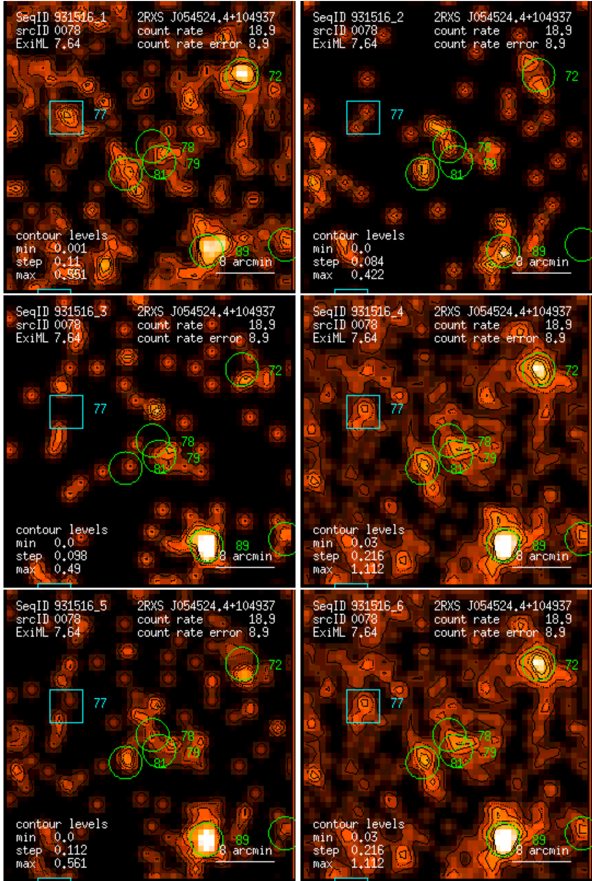
Figure 78: RASS 931516: detection 0078: band rate images, Gaussian filter: (1) PSPC channels 11 – 41, (2) 52 – 90, (3) 91 – 201, (4) 11 – 235, (5) 52 – 201, (6) 11 – 201. Broad band rates in counts/ks. Band rate contour levels in counts/ks/arcmin 2 .
