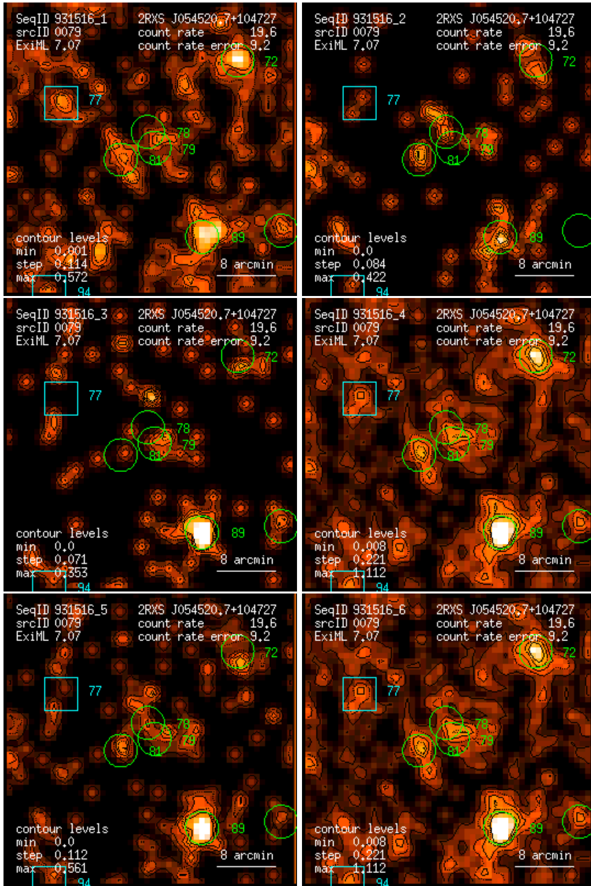
Figure 79: RASS 931516: detection 0079: band rate images, Gaussian filter: (1) PSPC channels 11 – 41, (2) 52 – 90, (3) 91 – 201, (4) 11 – 235, (5) 52 – 201, (6) 11 – 201. Broad band rates in counts/ks. Band rate contour levels in counts/ks/arcmin 2 .
