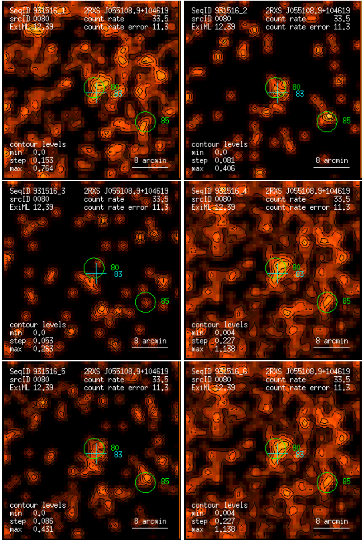
Figure 80: RASS 931516: detection 0080: band rate images, Gaussian filter: (1) PSPC channels 11 – 41, (2) 52 – 90, (3) 91 – 201, (4) 11 – 235, (5) 52 – 201, (6) 11 – 201. Broad band rates in counts/ks. Band rate contour levels in counts/ks/arcmin 2 .
