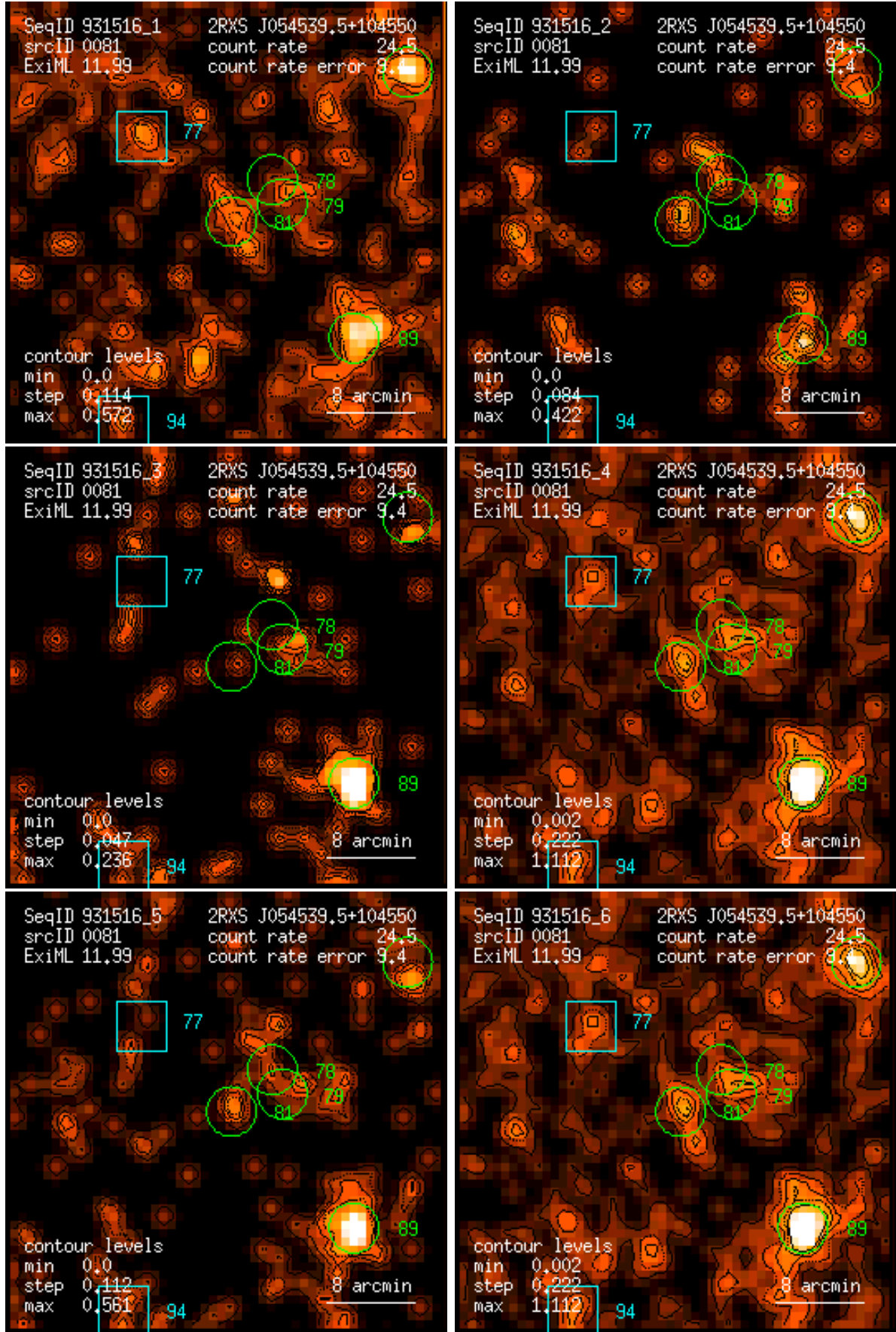
Figure 81: RASS 931516: detection 0081: band rate images, Gaussian filter: (1) PSPC channels 11 – 41, (2) 52 – 90, (3) 91 – 201, (4) 11 – 235, (5) 52 – 201, (6) 11 – 201. Broad band rates in counts/ks. Band rate contour levels in counts/ks/arcmin 2 .
