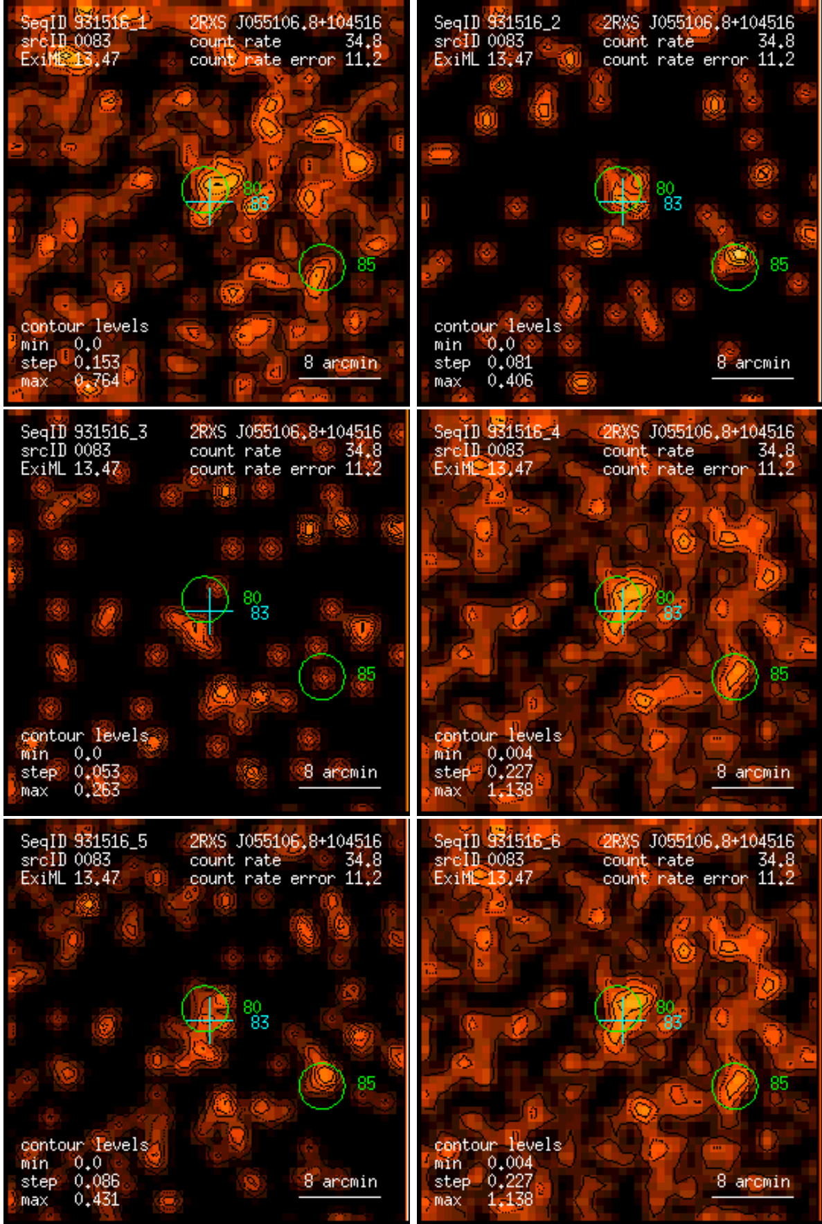
Figure 83: RASS 931516: detection 0083: band rate images, Gaussian filter: (1) PSPC channels 11 – 41, (2) 52 – 90, (3) 91 – 201, (4) 11 – 235, (5) 52 – 201, (6) 11 – 201. Broad band rates in counts/ks. Band rate contour levels in counts/ks/arcmin 2 .
