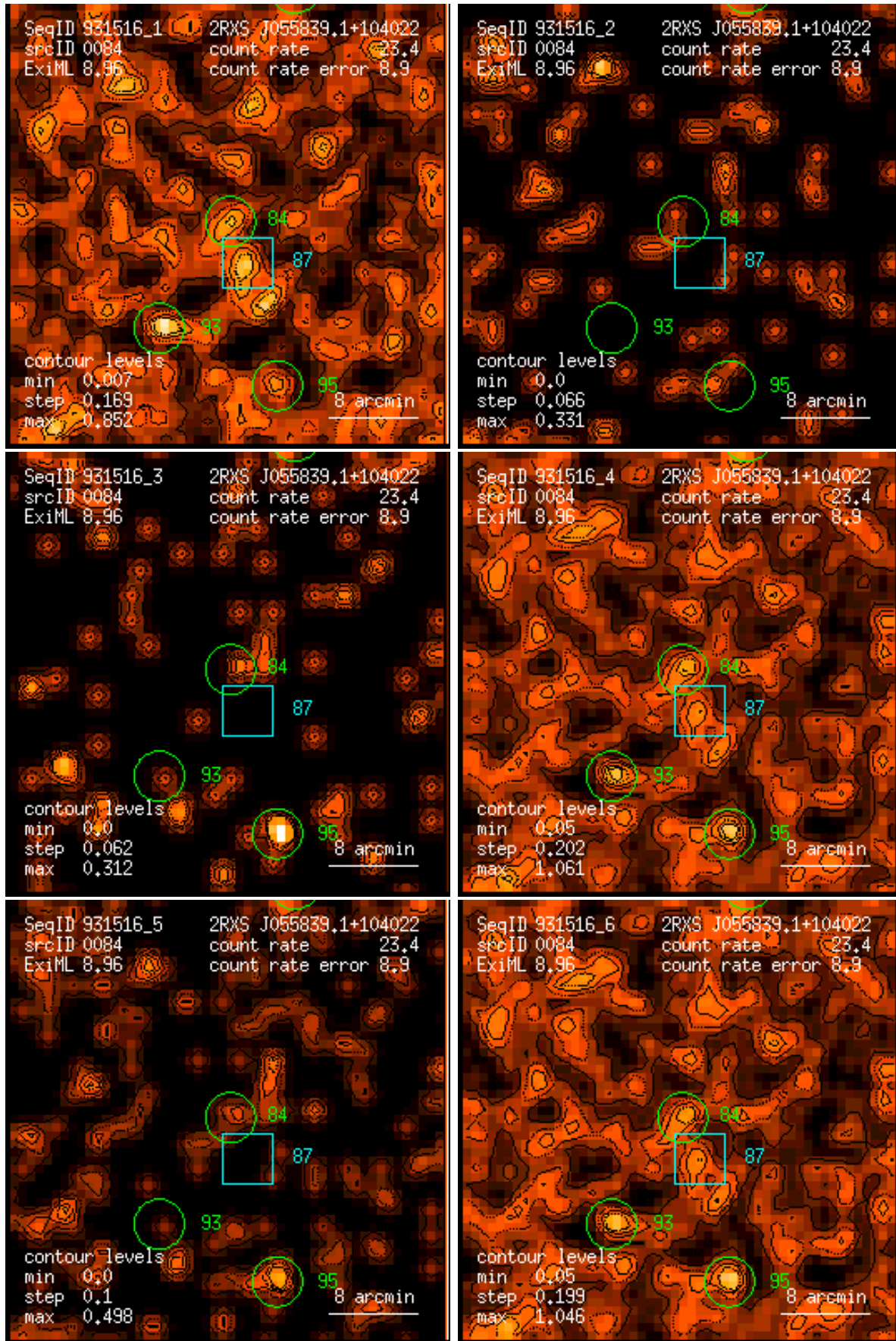
Figure 84: RASS 931516: detection 0084: band rate images, Gaussian filter: (1) PSPC channels 11 – 41, (2) 52 – 90, (3) 91 – 201, (4) 11 – 235, (5) 52 – 201, (6) 11 – 201. Broad band rates in counts/ks. Band rate contour levels in counts/ks/arcmin 2 .
