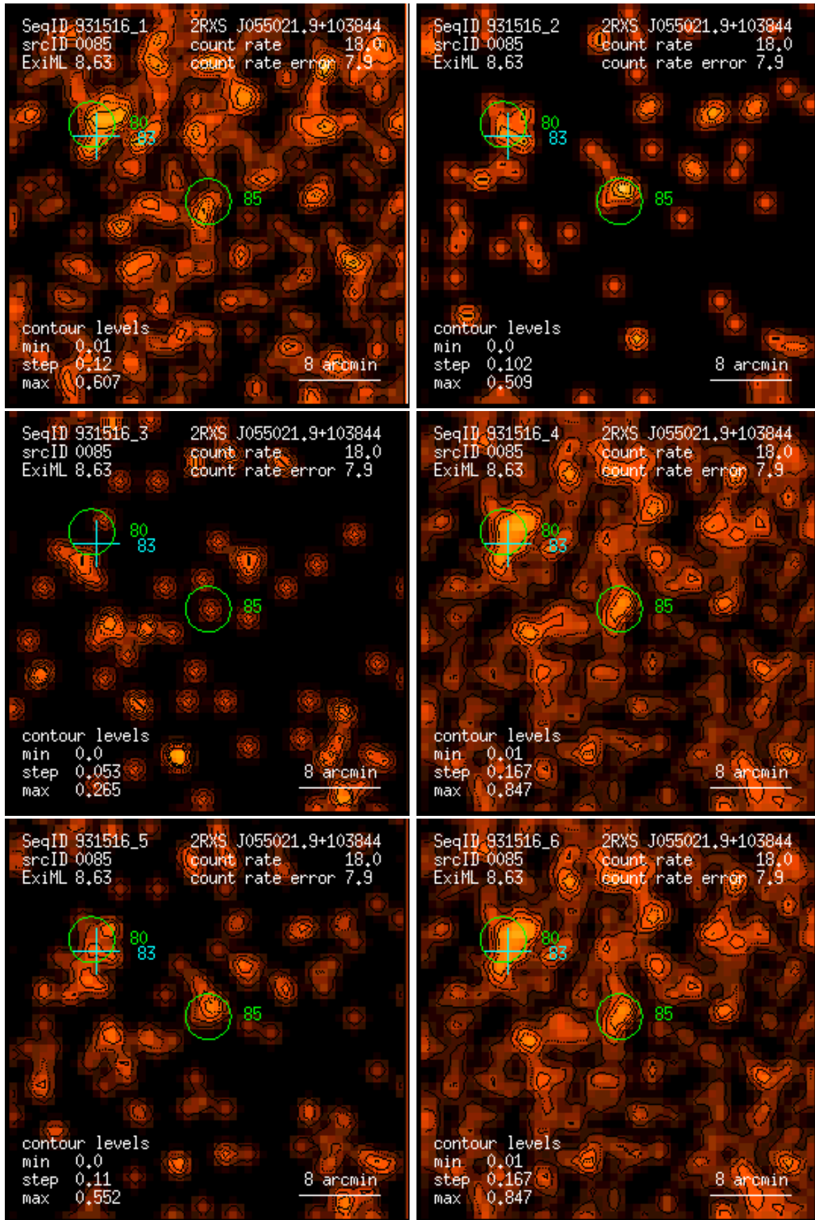
Figure 85: RASS 931516: detection 0085: band rate images, Gaussian filter: (1) PSPC channels 11 – 41, (2) 52 – 90, (3) 91 – 201, (4) 11 – 235, (5) 52 – 201, (6) 11 – 201. Broad band rates in counts/ks. Band rate contour levels in counts/ks/arcmin 2 .
