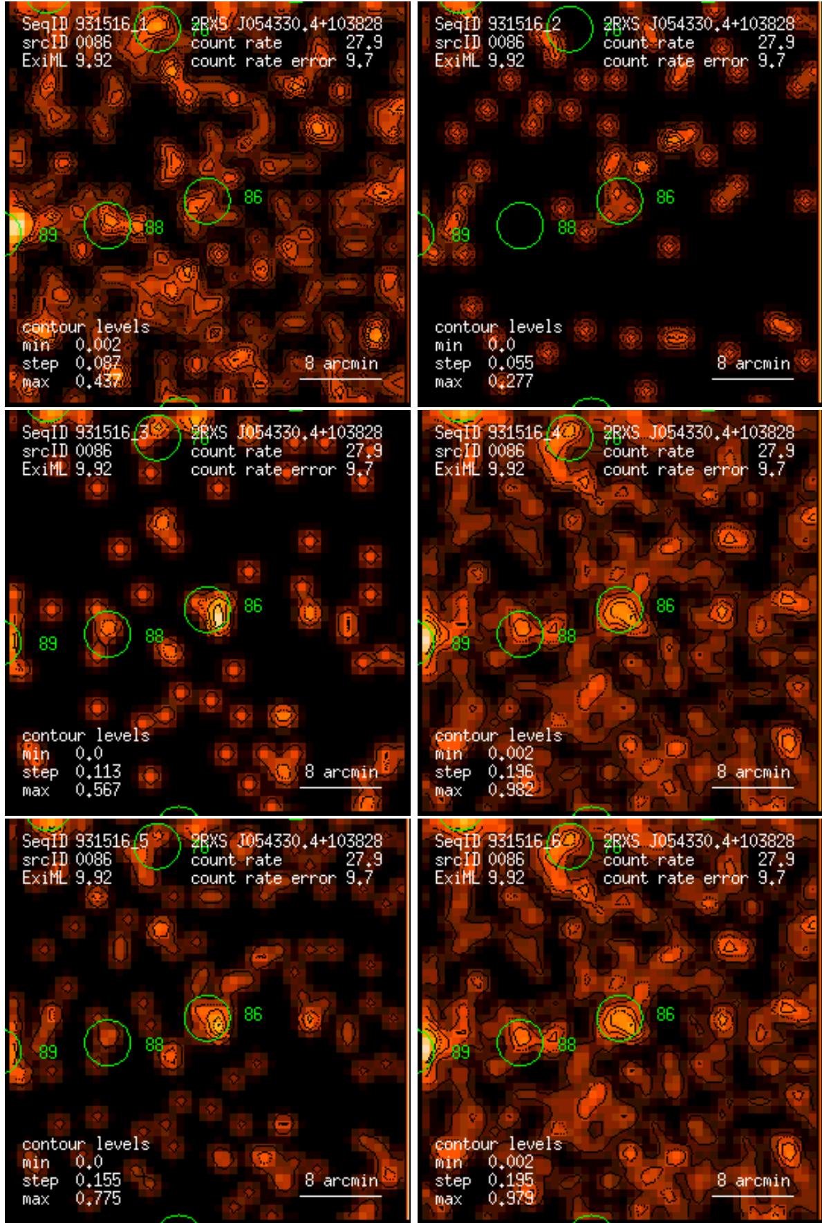
Figure 86: RASS 931516: detection 0086: band rate images, Gaussian filter: (1) PSPC channels 11 – 41, (2) 52 – 90, (3) 91 – 201, (4) 11 – 235, (5) 52 – 201, (6) 11 – 201. Broad band rates in counts/ks. Band rate contour levels in counts/ks/arcmin 2 .
